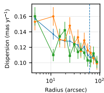
NGC 7099
