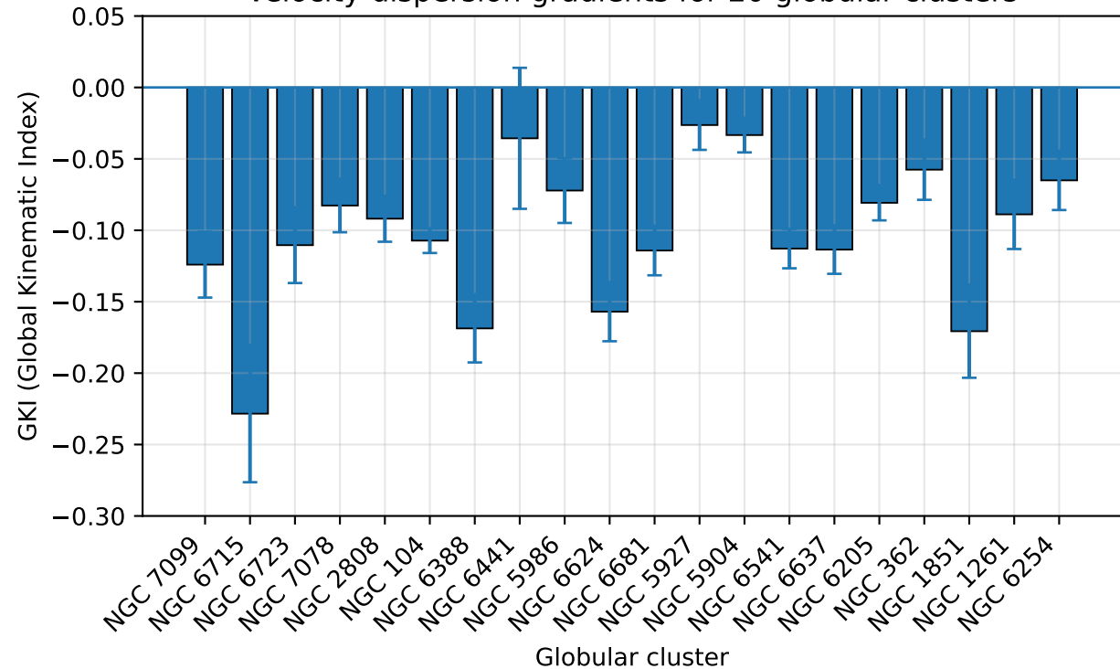
Velocity-dispersion gradients for 20 globular clusters
