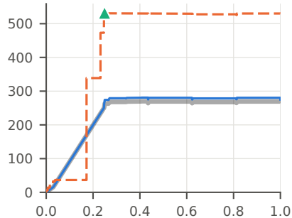
heap churn
