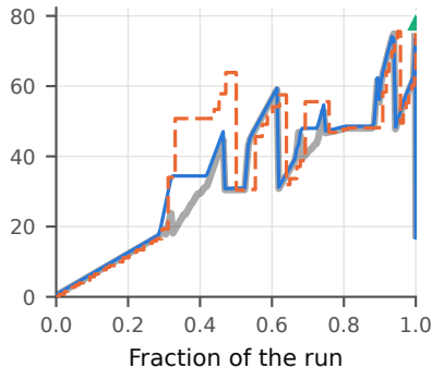
SQLite
