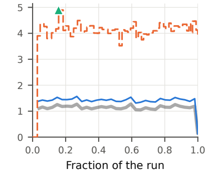
heap churn
