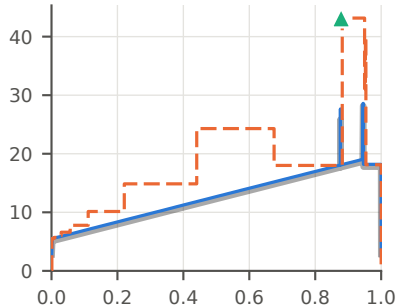
SQLite
