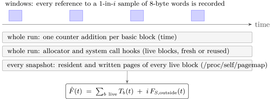
Figure 5: Windowed sampling. References are checked only inside windows (shaded). Time, live blocks and page information are tracked for the whole run. T_b is the touched bytes of block b (resident bytes for a fresh block, bytes on written pages for a reused block), and F_{S, \text{outside}} is the selected bytes outside all blocks.
