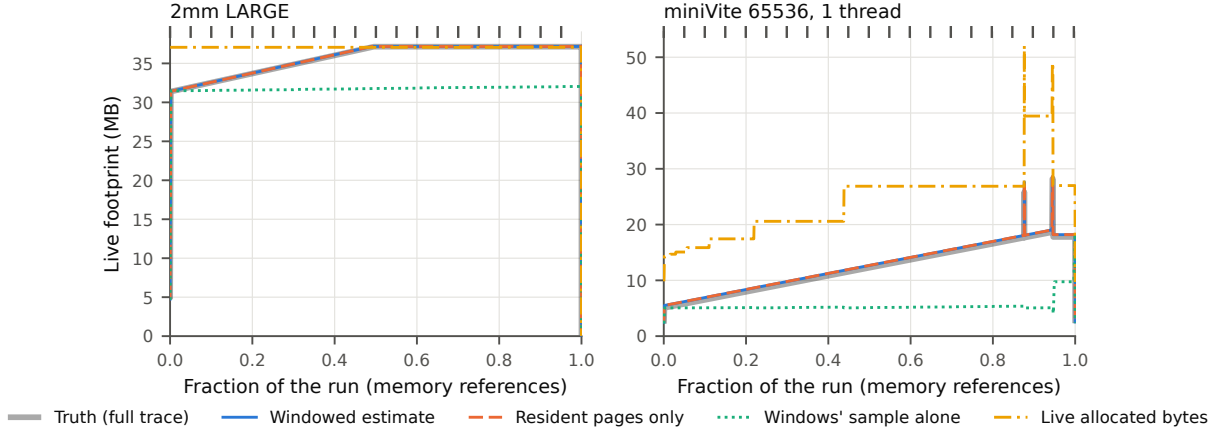
Figure 6: Live footprint over the run with 5% of the run watched (20 windows, marked at the top) and 1 in 100 words selected. On 2mm LARGE the windowed estimate and residency alone coincide with the truth.
