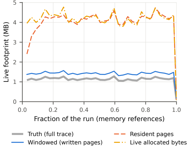
Figure 8: Heap churn with a quarter of each block written, 5% of the run watched. Resident pages include memory that freed blocks touched, whereas the pages written since each block’s allocation follow the truth to within whole pages.
