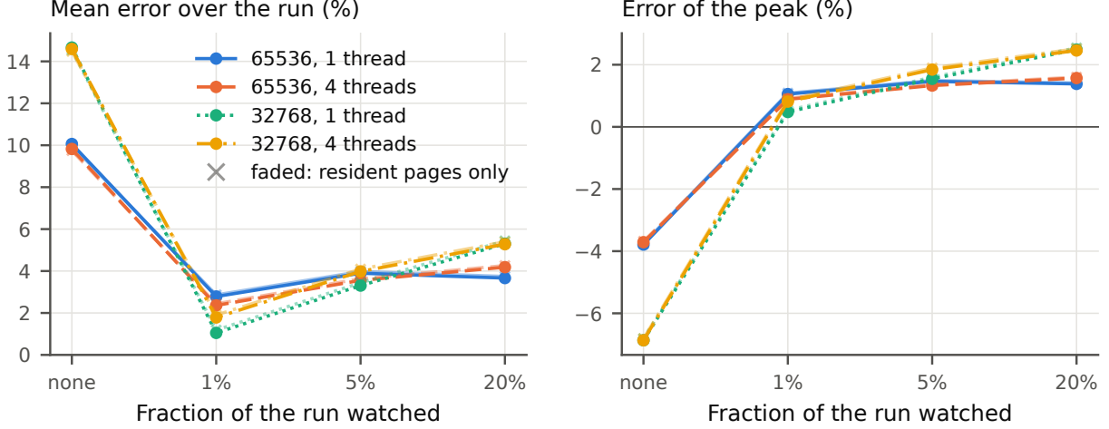
Figure 7: miniVite: windowed estimate error against the fraction of the run watched, with 1 in 100 words. Faded lines are residency alone, without written pages.
