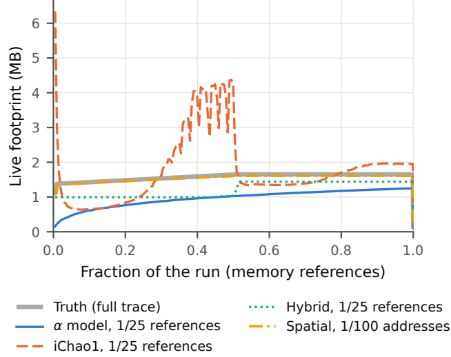
Figure 3: Live footprint of 2mm MEDIUM (held out from training) over the run, against estimates from 1-in-25 samples of references and from a 1-in-100 sample of words. The word sample follows the truth closely, whereas the estimates from sampled references overshoot, undershoot or lag.
