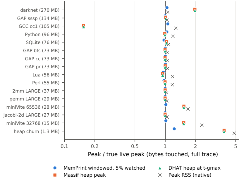
Figure 1: Peaks relative to the true live peak (bytes touched, complete recording, given in brackets): the windowed estimate at 5% watched, Massif’s heap peak, DHAT’s heap at its global maximum, and the native peak resident memory. Workloads are sorted by true peak; the markers of each workload are spread vertically so that equal values stay visible.
