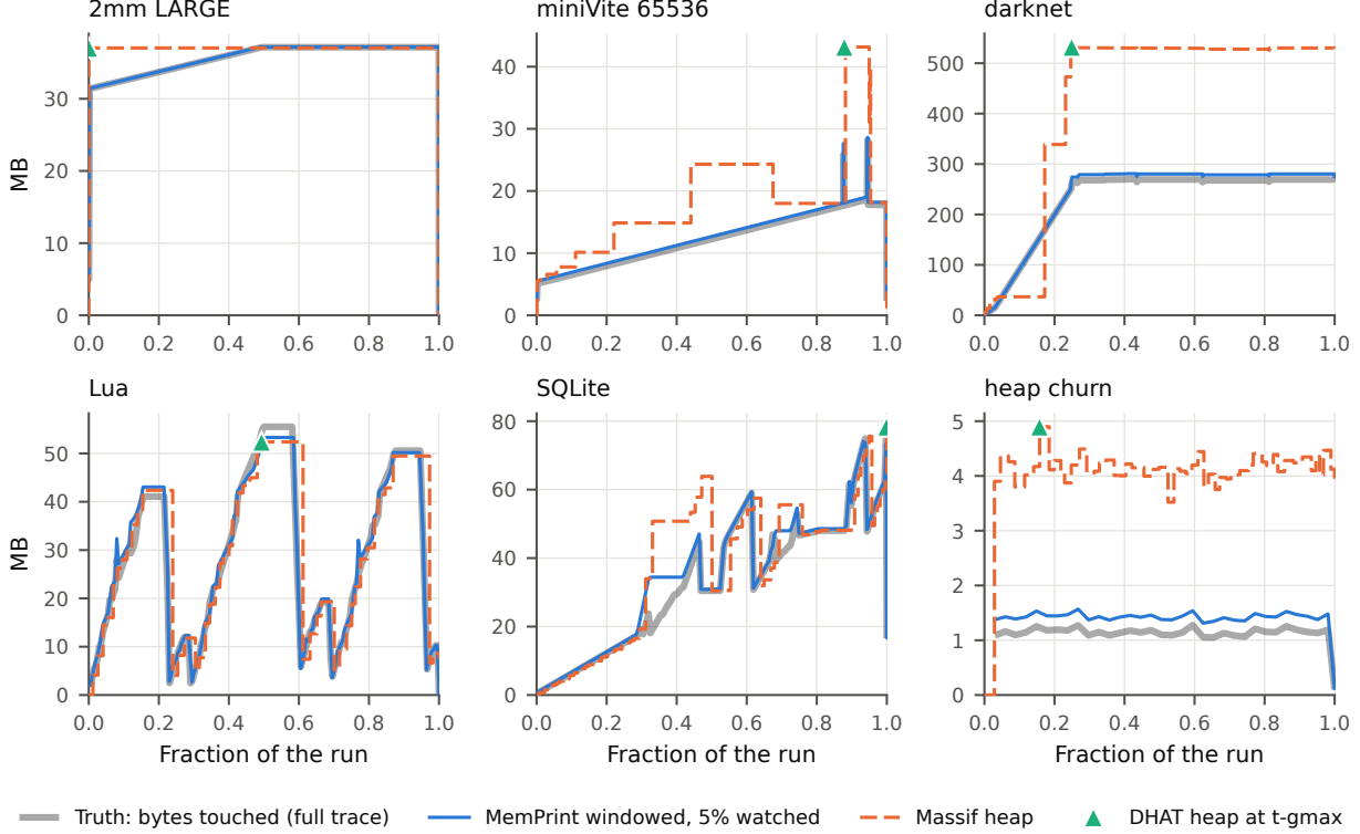
Figure 2: Live footprint over the run: the truth (bytes touched), the windowed estimate at 5% watched, Massif’s heap, and DHAT’s heap at its global maximum, placed at the moment it occurs. Time is a fraction of the run, counted in memory references for MemPrint and in instructions for Valgrind.
