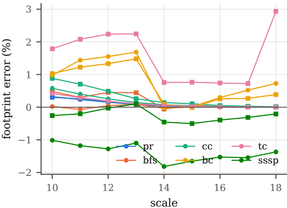
C++ interpreter footprint (○ uniform, □ Kronecker)
