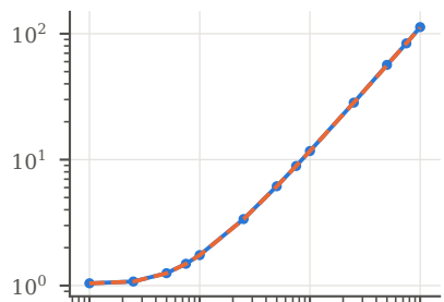
trisolv (2.5% off)
