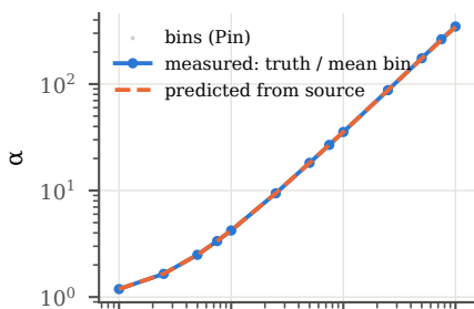
jacobi-2d (0.2% off)
