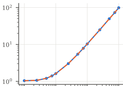
floyd-warshall (12.8% off)
