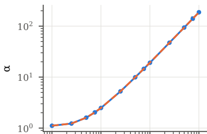
nussinov (14.3% off)
