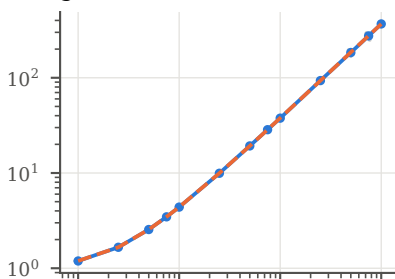
lu (0.2% off)
