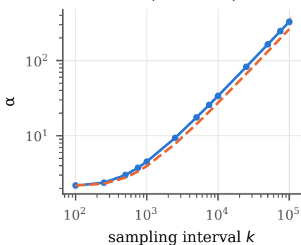
nussinov (14.3% off)
