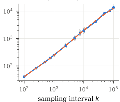
trisolv (2.5% off)
