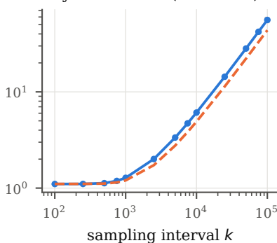
floyd-warshall (12.8% off)
