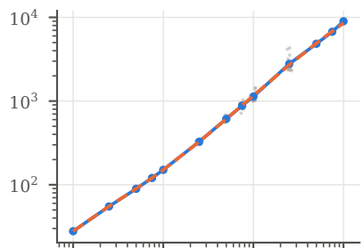
cholesky (0.3% off)
