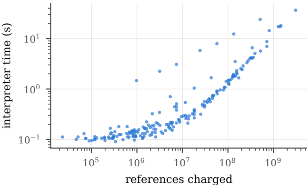
(a) Cost of the C interpreter, 27 kernels \times 7 sizes
