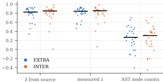
(a) Does descriptor distance rank transfer error?
