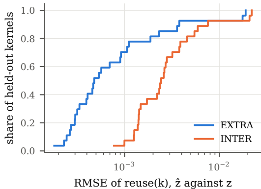
(b) Accuracy of \hat{z}
