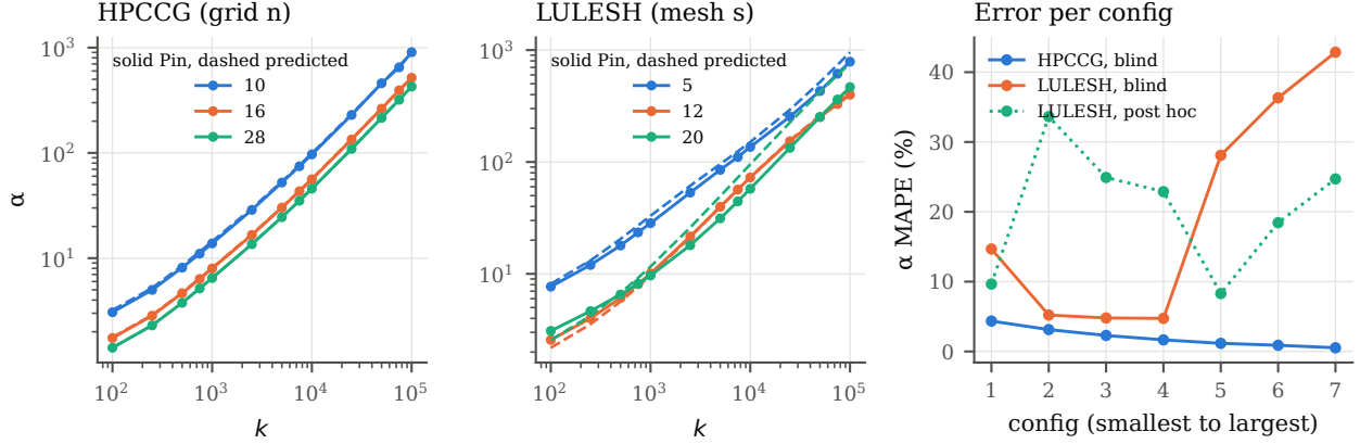
Figure 28: Blind test. Left and middle: \alpha against the interval, traced (solid) and predicted before tracing (dashed), for three configs of each program. Right: \alpha MAPE per config.
