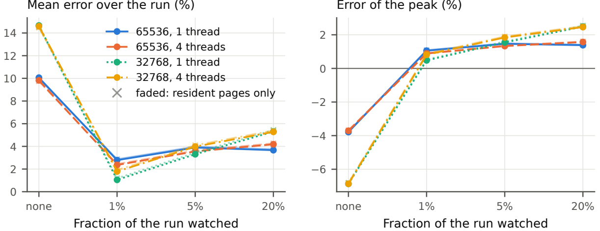
Figure 5: miniVite: windowed estimate error against the fraction of the run watched, with 1 in 100 words. Faded lines are residency alone, without written pages.
