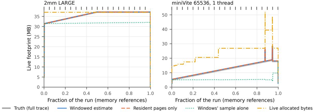
Figure 4: Live footprint over the run with 5% of the run watched (20 windows, marked at the top) and 1 in 100 words selected. On 2mm LARGE the windowed estimate and residency alone coincide with the truth.
