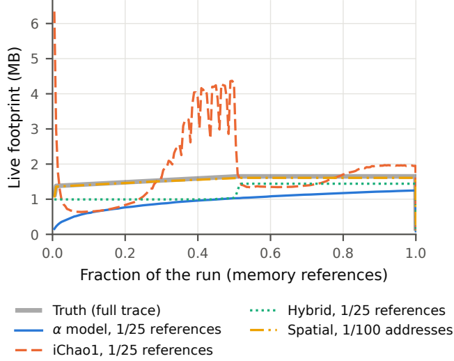
Figure 1: Live footprint of 2mm MEDIUM (held out from training) over the run, against estimates from 1-in-25 samples of references and from a 1-in-100 sample of words. The word sample follows the truth closely, whereas the estimates from sampled references overshoot, undershoot or lag.
