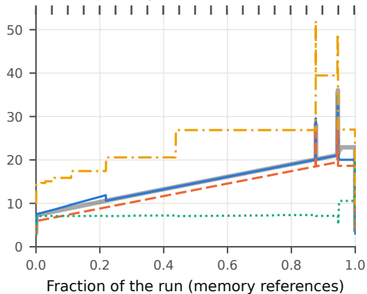
miniVite 65536, 1 thread
