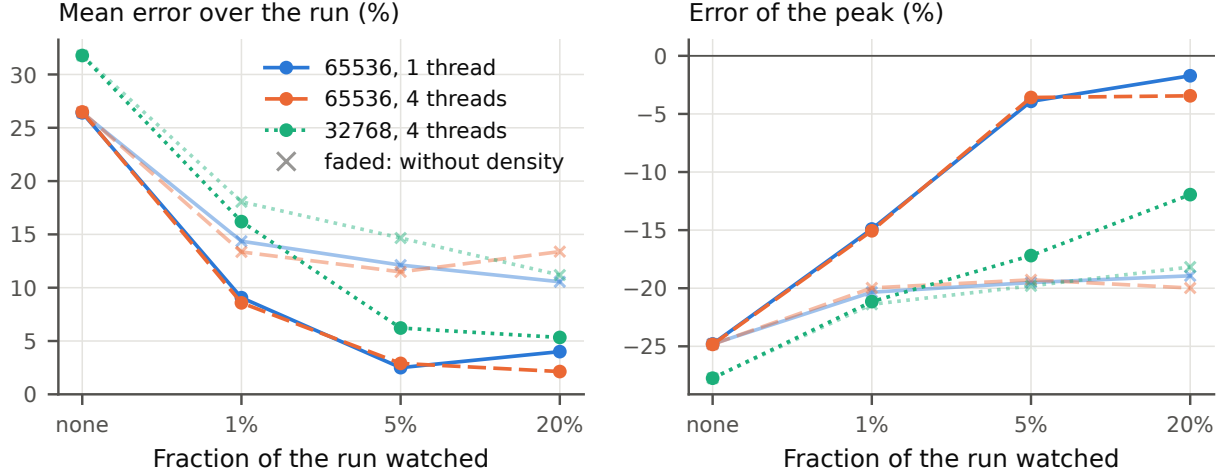
Figure 5: miniVite: windowed estimate error against the fraction of the run watched, with 1 in 100 chunks. Faded lines are the same estimate without the density correction.
