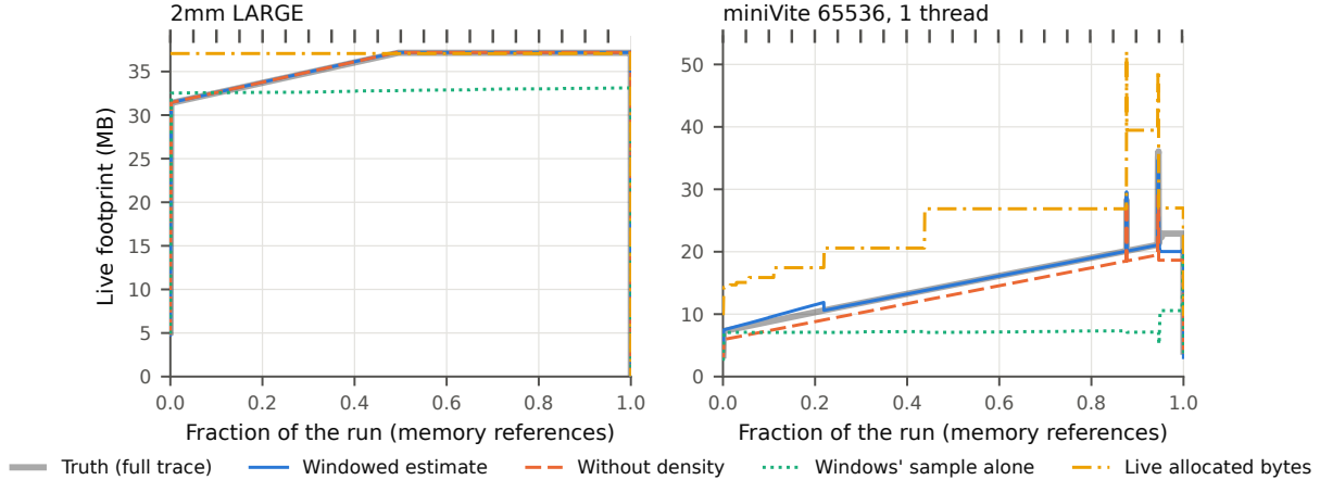
Figure 4: Live footprint over the run with 5% of the run watched (20 windows, marked at the top) and 1 in 100 chunks selected. On 2mm LARGE the windowed estimate and the estimate without density coincide with the truth.
