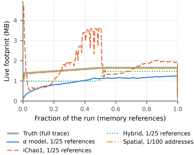
Figure 1: Live footprint of 2mm MEDIUM (held out) over the run, against estimates from 1-in-25 reference samples and from 1-in-100 address samples. The address sample tracks the truth closely, while the reference sampling estimators overshoot, undershoot or lag.
