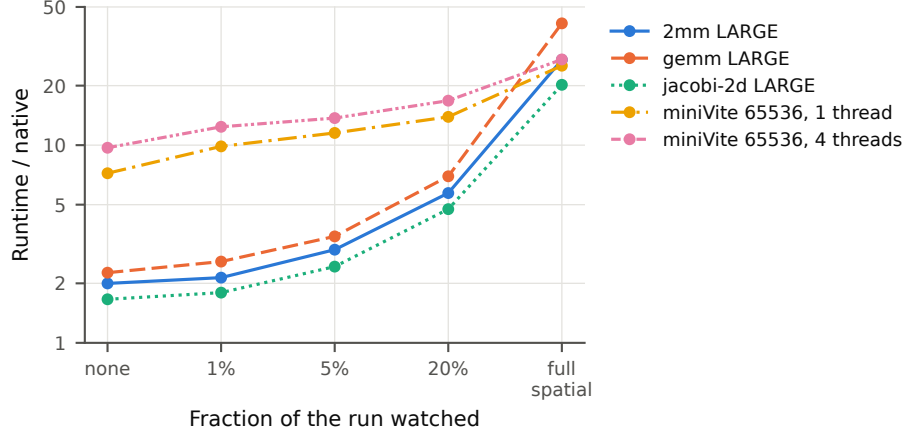
Figure 6: Runtime relative to native against the fraction of the run watched, with full address sampling for comparison (logarithmic scale).
