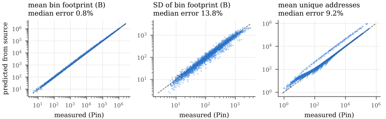
Figure 8: The three moments of (3), predicted from source against measured, for every kernel, config and interval (2,457 points).
