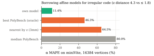
Figure 16: Errors on miniVite of its own model and of borrowed PolyBench models.
