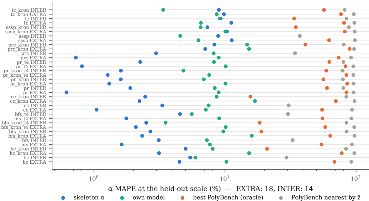
GAP: predicting from the skeleton against borrowing a model
