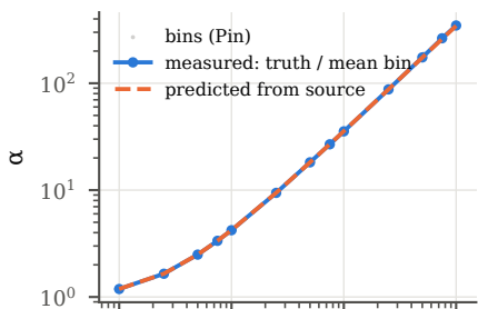
jacobi-2d (0.2% off)
