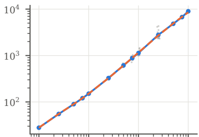
cholesky (0.3% off)
