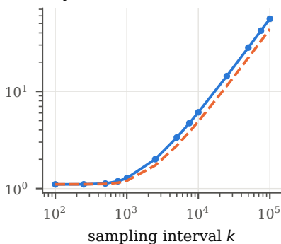
floyd-warshall (12.8% off)
