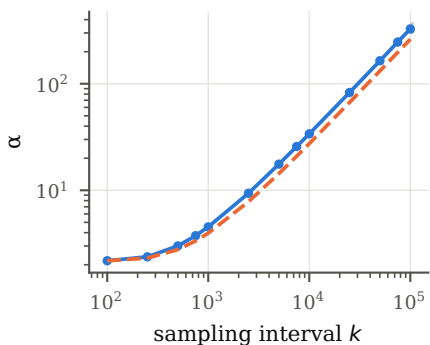
nussinov (14.3% off)
