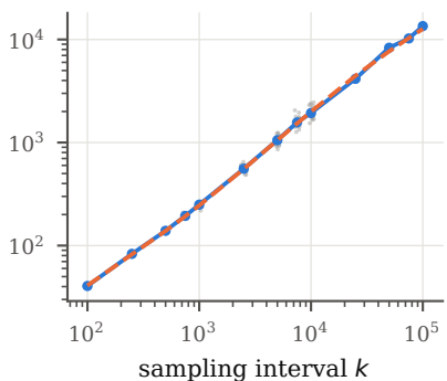
trisolv (2.5% off)
