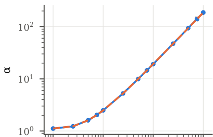
nussinov (14.3% off)
