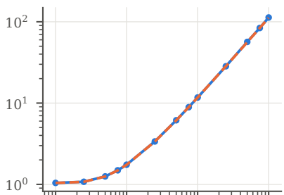
trisolv (2.5% off)
