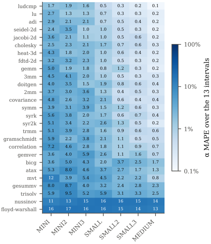
Static \alpha error per kernel and input size
