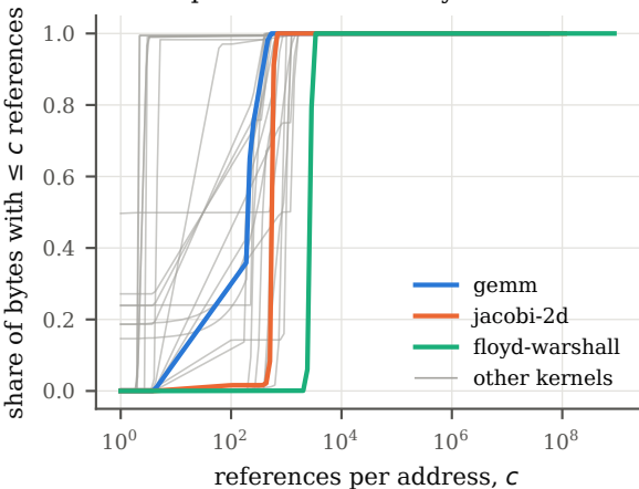
Static spectra of the 27 PolyBench kernels (MEDIUM)
