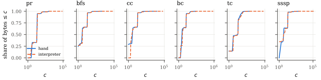
Figure 25: Cumulative spectra at scale 12 (uniform): hand skeleton against the interpreter.
