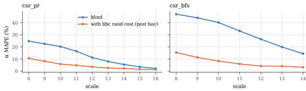
Figure 21: \alpha MAPE per scale of the interpreter on two irregular C programs, blind and with the libc rand() cost.
