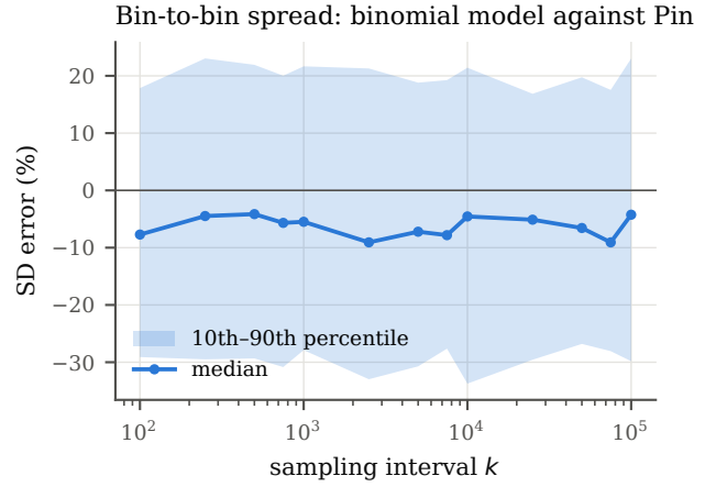
Figure 10: Signed error of the predicted standard deviation of the bin footprint, by interval.
