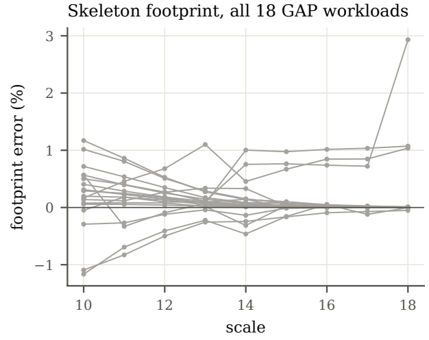
Figure 18: Skeleton footprint error at every scale, all GAP workloads.
