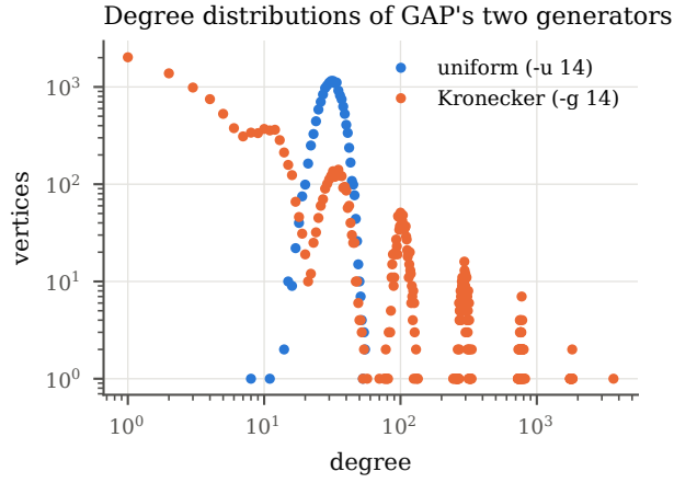
Figure 17: Degree distributions of the graphs drawn from GAP's two generators at scale 14.
