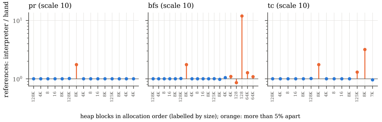
Figure 26: References to each heap block, interpreter over hand skeleton, at scale 10.
