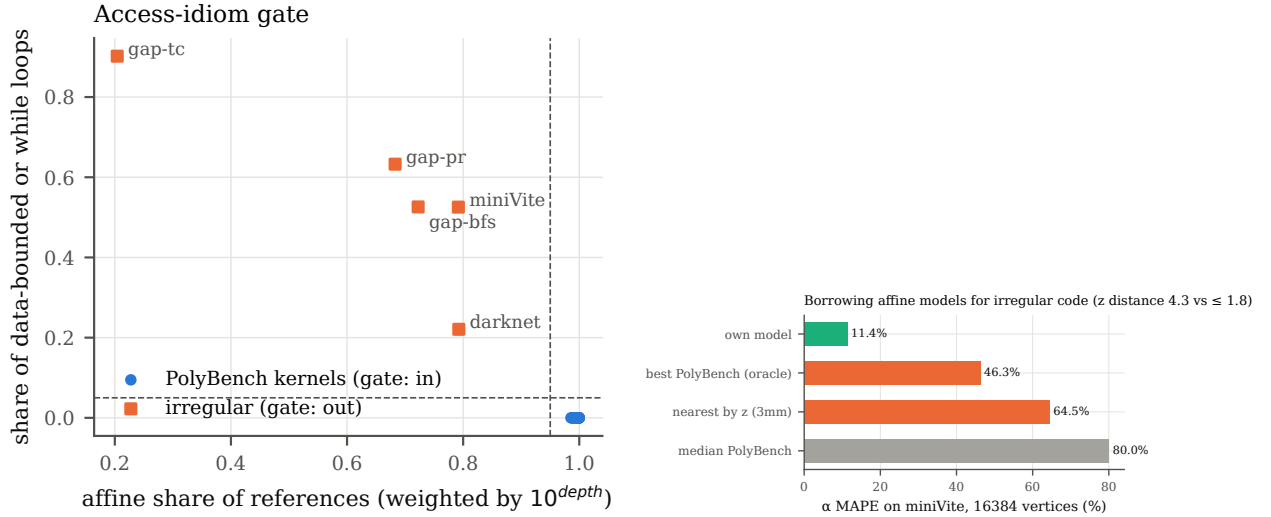
Figure 15: Affine share against the share of data-bounded or while loops. Dashed: the gate's thresholds.
