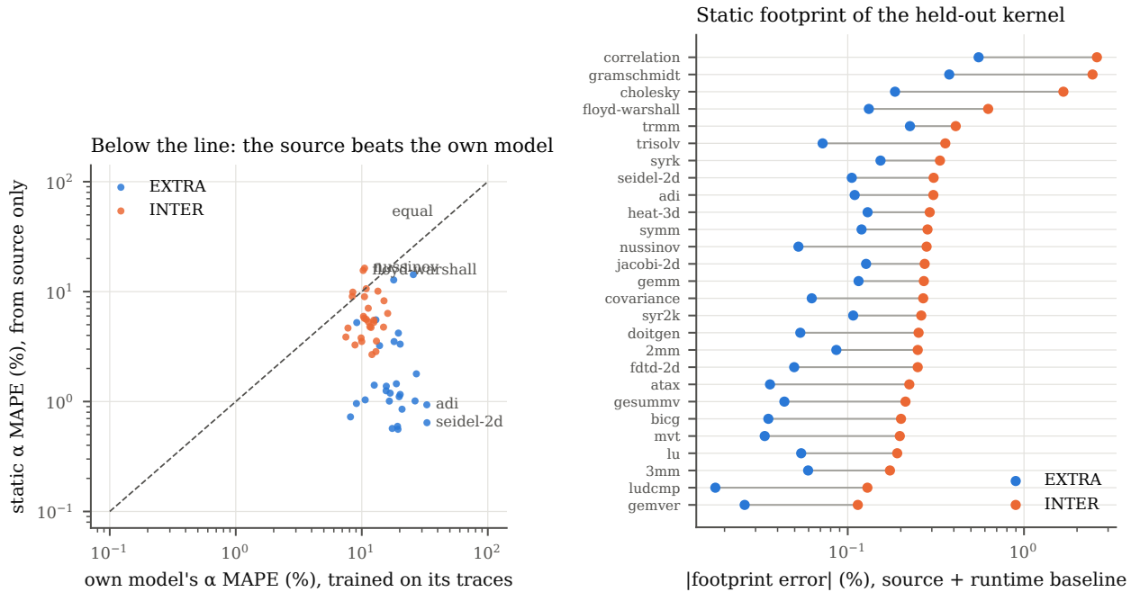
Figure 5: Static \alpha error (from the source only) against the own model’s error (trained on the kernel’s traces), per kernel and split.
