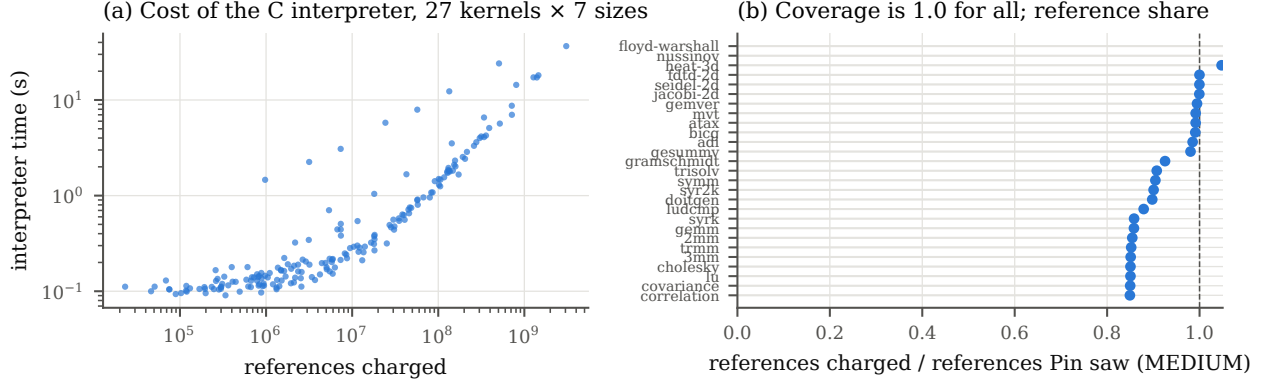
Figure 14: (a) Interpreter time per kernel and config. (b) References the interpreter charges as a share of those Pin records, at MEDIUM. Coverage is 1.0 for every kernel.
