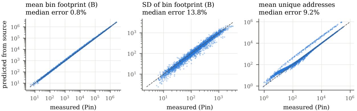
Figure 8: The three moments of (3), predicted from source against measured, for every kernel, config and interval (2,457 points).
