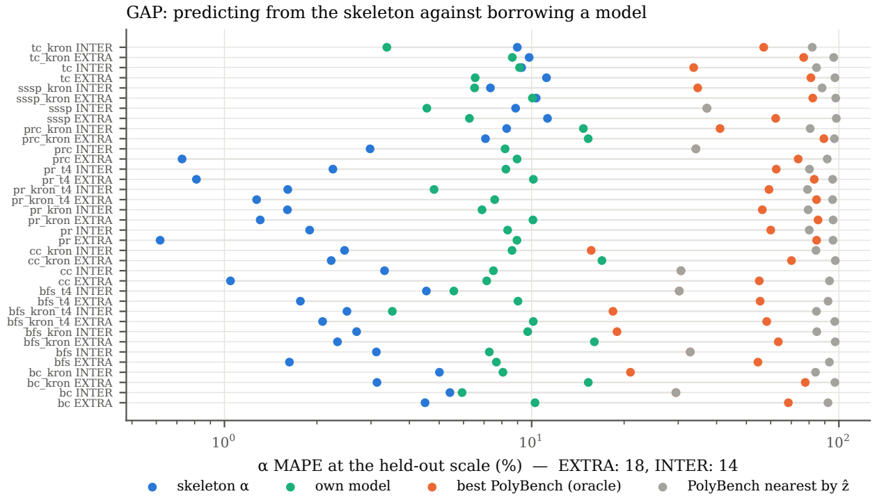
Figure 19: GAP: \alpha error of the skeleton, the workload's own model and the borrowed PolyBench models, per workload and split.
