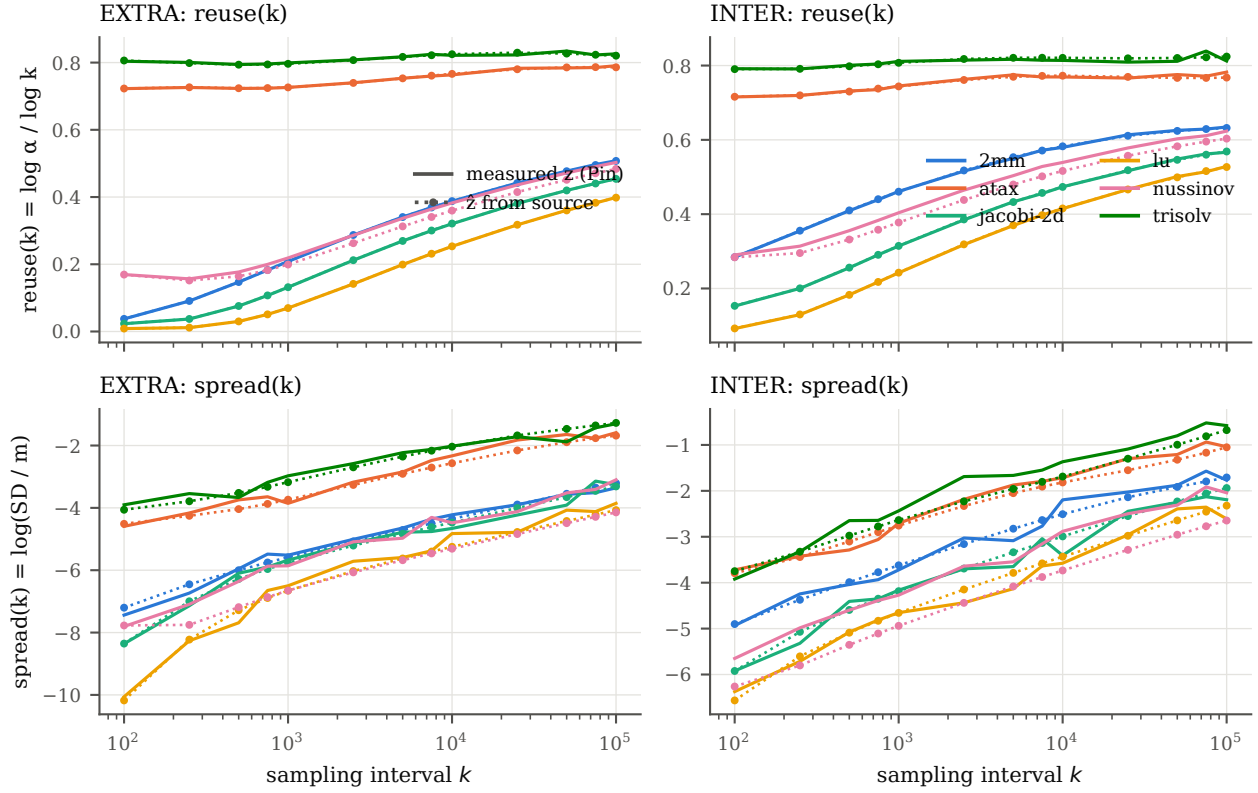
Figure 13: The two parts of the descriptor, measured (solid) and predicted from source (dotted), for six kernels.
