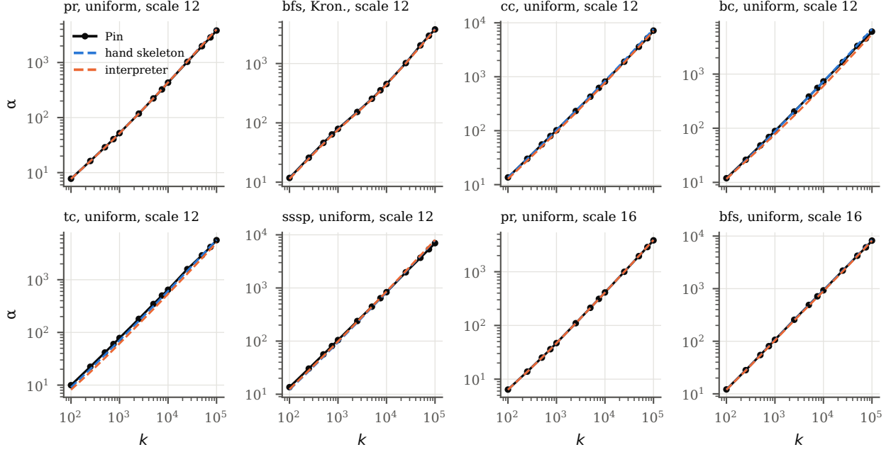
Figure 23: \alpha against the interval: Pin, the hand skeleton and the interpreter, for eight workload-scale pairs.
