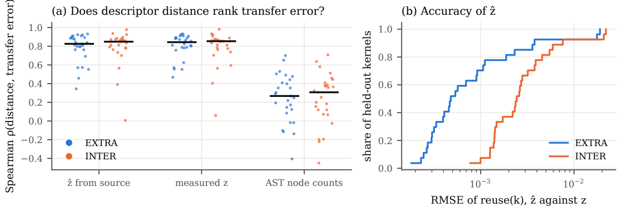
Figure 12: (a) Spearman \rho between descriptor distance and transfer error, one dot per held-out kernel (bars: medians). (b) Cumulative distribution of the RMSE between \hat{z} and z on reuse( k ).
