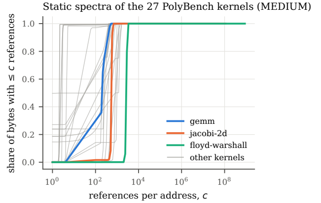
Figure 11: Cumulative static spectra at MEDIUM: the share of bytes referenced at most c times.
