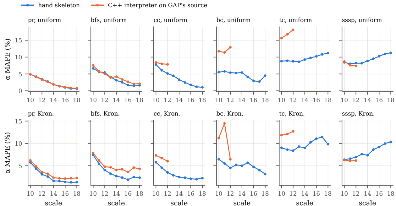
Figure 22: \alpha MAPE per scale: hand skeleton against the C++ interpreter on GAP’s source, six kernels, uniform (top) and Kronecker (bottom) graphs.
