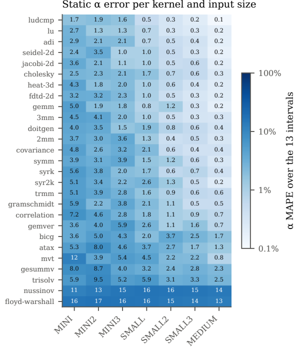
Figure 9: Static \alpha MAPE per kernel and input size (baseline fitted without the kernel).
