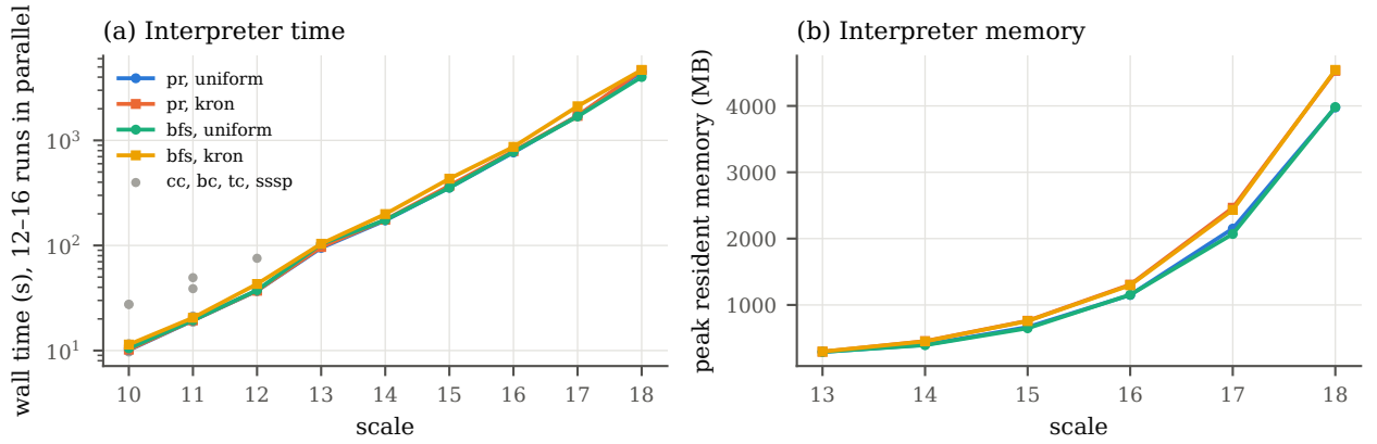
Figure 27: Wall time and peak memory of the C++ interpreter per scale.
