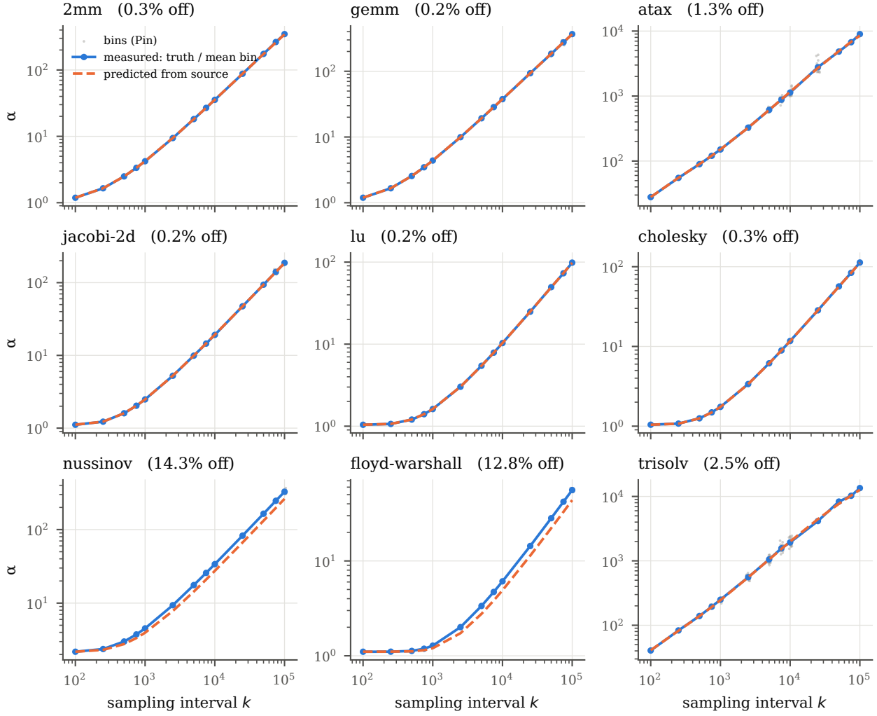
Figure 7: \alpha against the sampling interval at MEDIUM: every Pin bin (gray), the measured truth over the mean bin footprint (blue) and the prediction from the source (orange, dashed). The title gives the MAPE over the 13 intervals.
