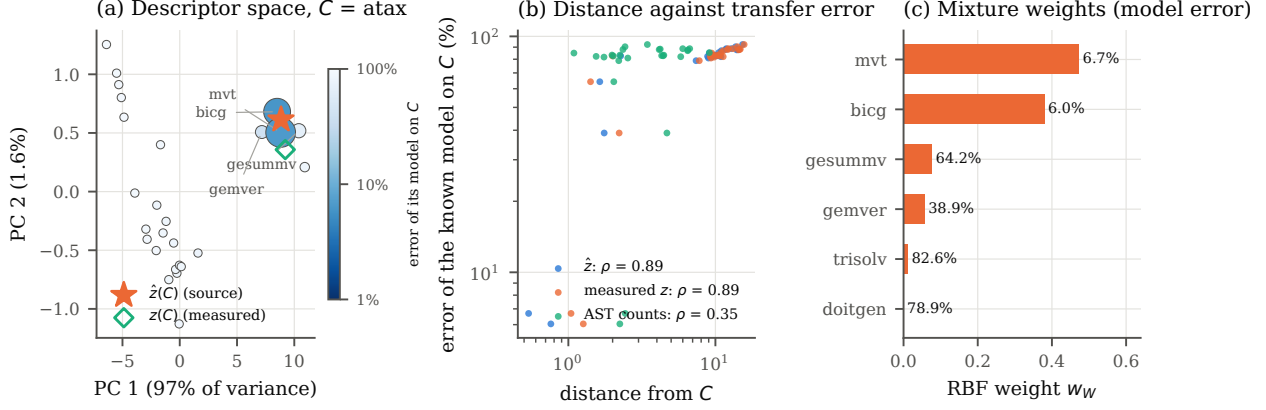
Figure 7: Borrowing for atax (EXTRA). (a) The 26 known kernels in the first two principal components of the standardised descriptors, coloured by the error of their model on atax and sized by their RBF weight; the star is atax’s descriptor predicted from source, the diamond its measured one. (b) Distance from atax against the error of each known model on atax, for the three distances, with Spearman’s \rho . (c) The six largest mixture weights, with each model’s error on atax.
