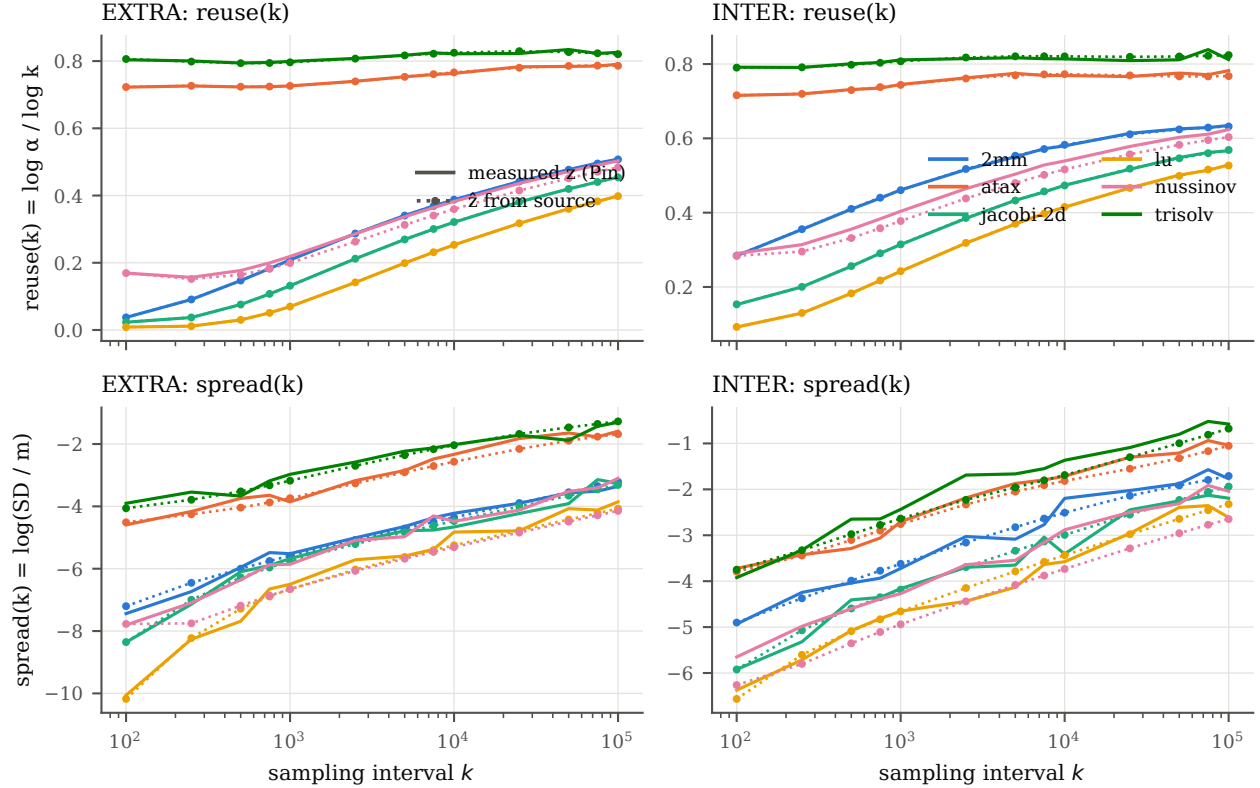
Figure 17: The two parts of the descriptor, measured (solid) and predicted from source (dotted), for six kernels.
