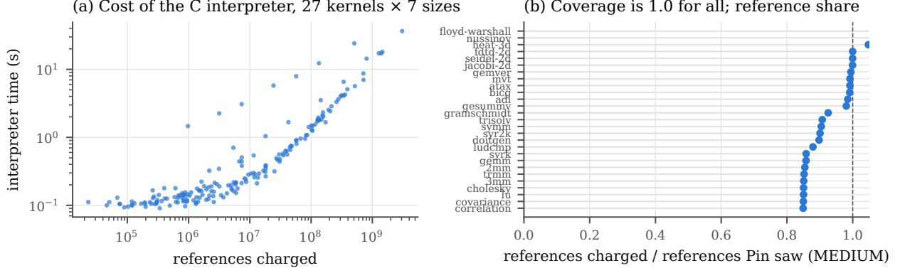
Figure 18: (a) Interpreter time per kernel and config. (b) References the interpreter charges as a share of those Pin records, at MEDIUM. Coverage is 1.0 for every kernel.
