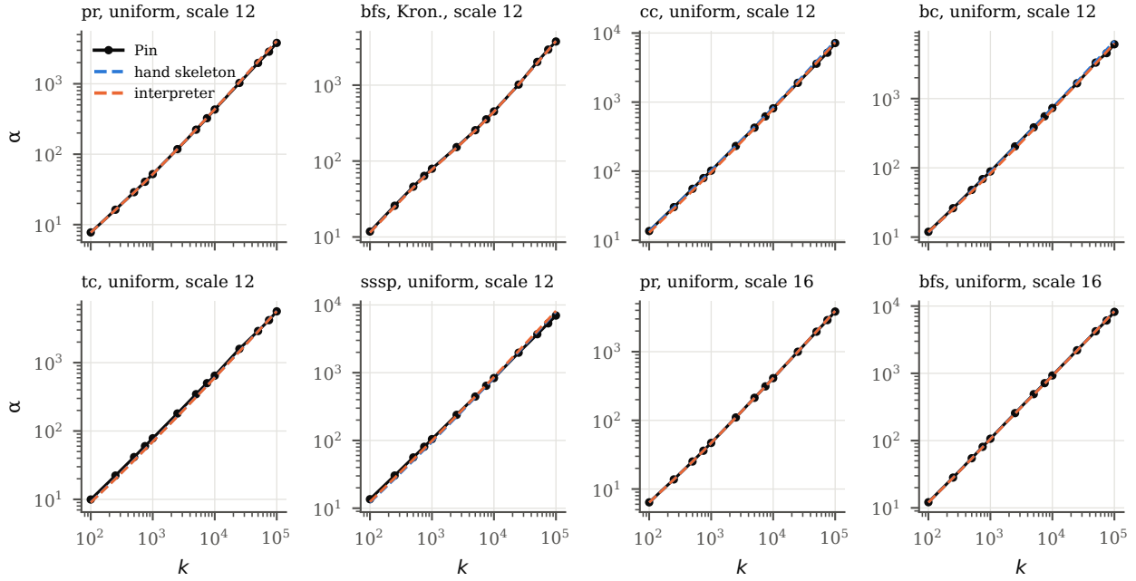
Figure 27: \alpha against the interval: Pin, the hand skeleton and the interpreter, for eight workload-scale pairs.
