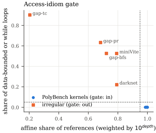
Figure 19: Affine share against the share of data-bounded or while loops. Dashed: the gate’s thresholds.
