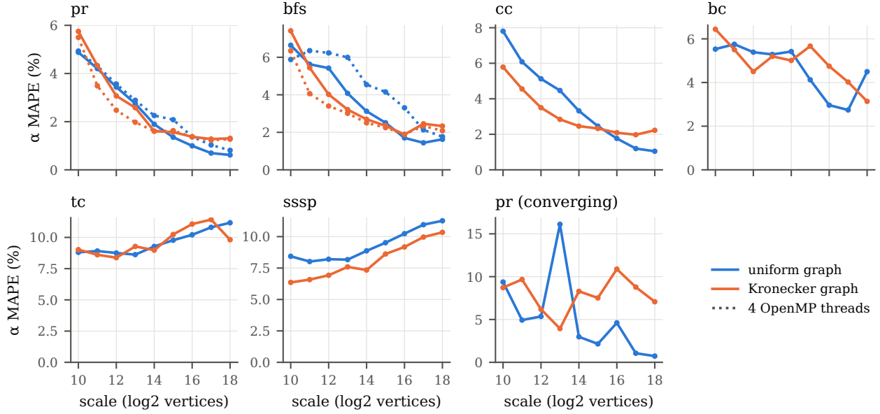
Figure 24: Skeleton \alpha MAPE at every scale, for the seven kernels, both graph families and (pr, bfs) 4 threads.
