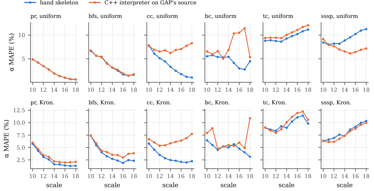
Figure 26: \alpha MAPE per scale: hand skeleton against the C++ interpreter on GAP's source, six kernels, uniform (top) and Kronecker (bottom) graphs.
