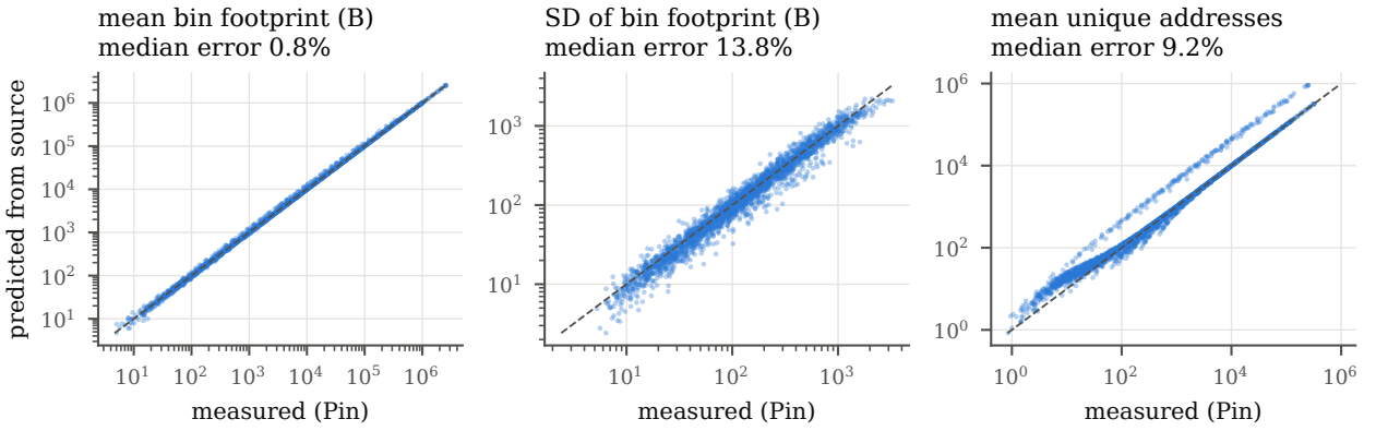
Figure 12: The three moments of (3), predicted from source against measured, for every kernel, config and interval (2,457 points).
