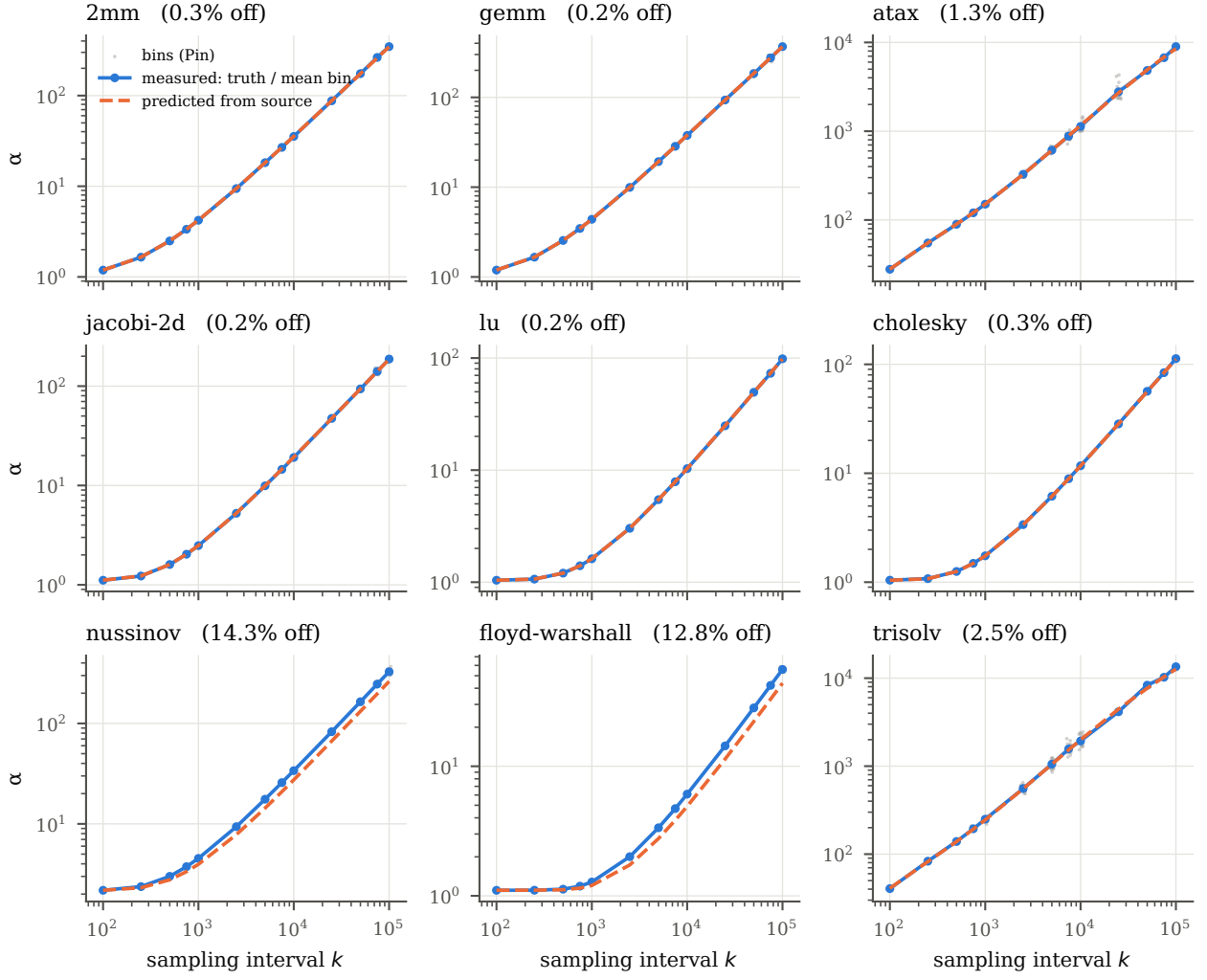
Figure 11: \alpha against the sampling interval at MEDIUM: every Pin bin (gray), the measured truth over the mean bin footprint (blue) and the prediction from the source (orange, dashed). The title gives the MAPE over the 13 intervals.
