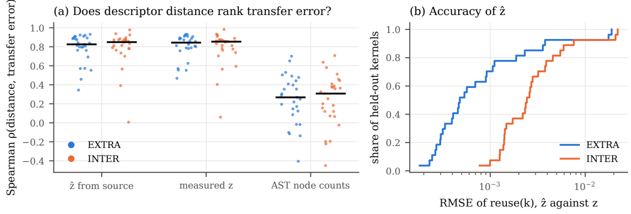
Figure 16: (a) Spearman \rho between descriptor distance and transfer error, one dot per held-out kernel (bars: medians). (b) Cumulative distribution of the RMSE between \hat{z} and z on \text{reuse}(k) .
