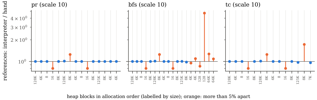
Figure 30: References to each heap block, interpreter over hand skeleton, at scale 10.
