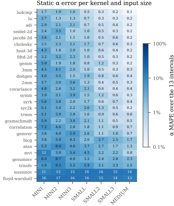
Figure 13: Static \alpha MAPE per kernel and input size (baseline fitted without the kernel).
