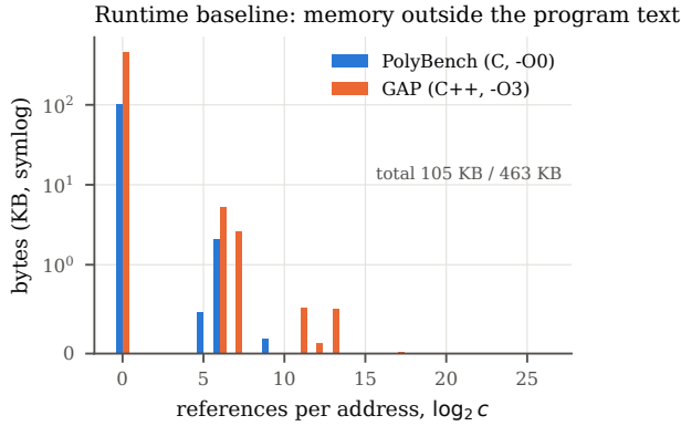
Figure 3: Runtime baselines fitted by NNLS: bytes per reference-count class.
