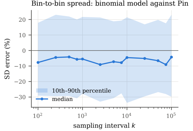
Figure 14: Signed error of the predicted standard deviation of the bin footprint, by interval.
