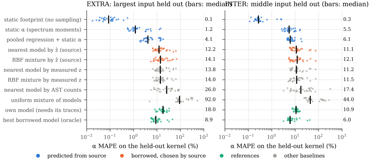
Figure 8: Leave-one-out MAPE of every method on each held-out kernel (dots; bars and numbers: medians). Blue: predicted from the source. Orange: a known model chosen by \hat{z} . Green: references that need the held-out kernel’s traces. Gray: other baselines.
