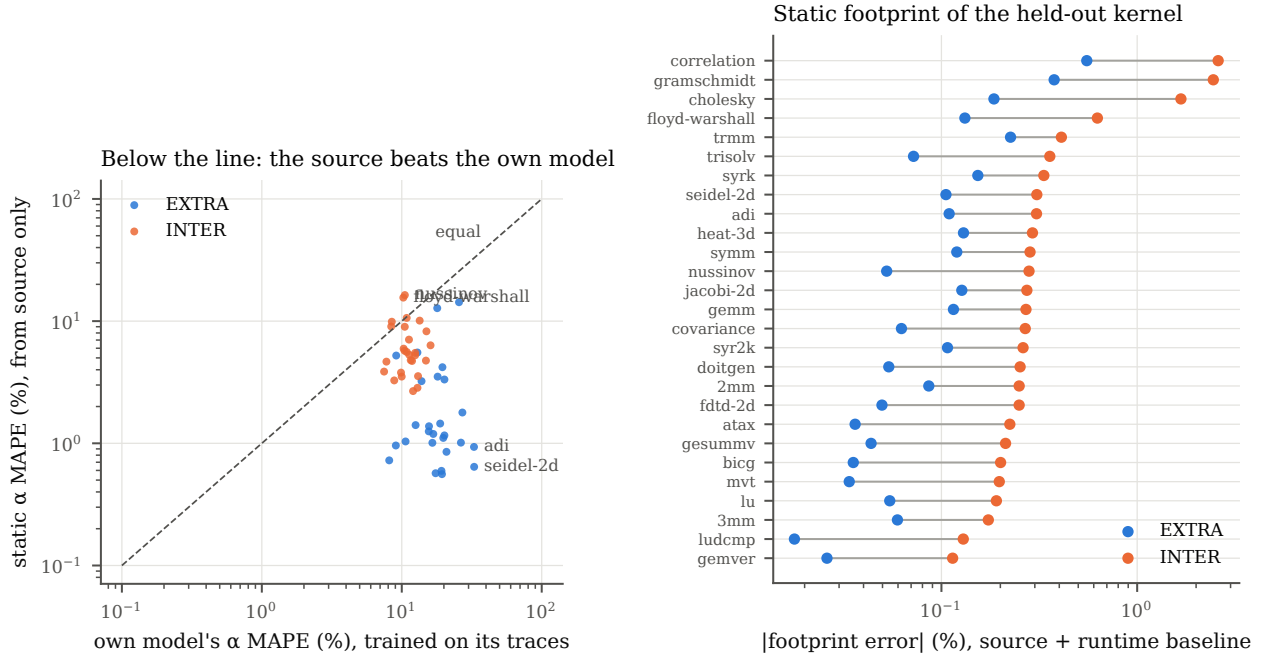
Figure 9: Static \alpha error (from the source only) against the own model’s error (trained on the kernel’s traces), per kernel and split.
