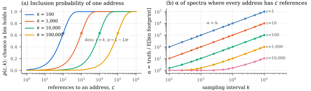
Figure 2: (a) The probability that a 1-in- k bin holds an address referenced c times, (2). (b) \alpha_k for spectra in which every 4-byte address is referenced exactly c times: \alpha_k \approx k/c while c \ll k , and \alpha_k \rightarrow 1 once c \gg k .
