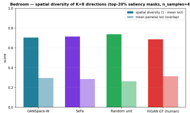
Figure 7. Spatial diversity baseline. Random unit directions are most spatially orthogonal; human-curated boundaries are least . Spatial-diversity score must be read alongside coverage — the two together pin a method on the trivia–meaning axis.
