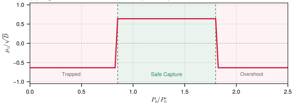
(a) Separatrix Traversal Window ( D = 2048 )
