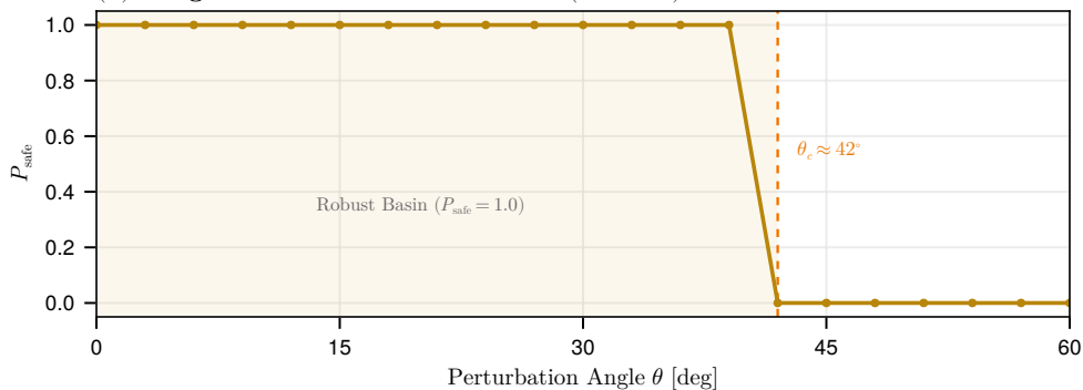
(b) Tangent Perturbation Robustness ( D = 2048 )
