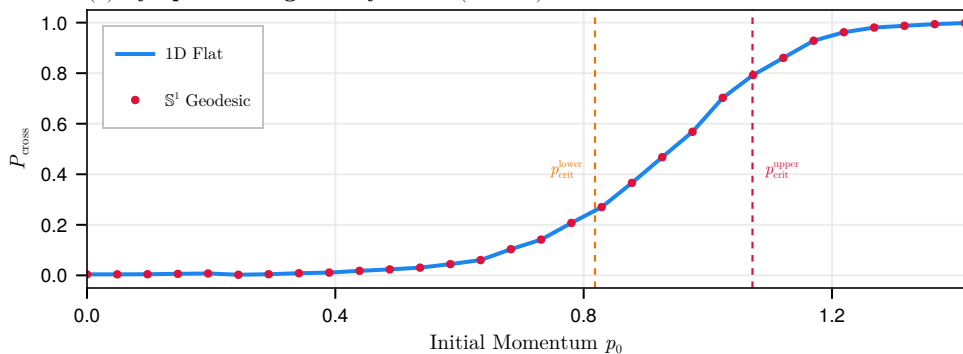
(c) Symplectic Degeneracy Proof ( S^1 \rightarrow 1D )
