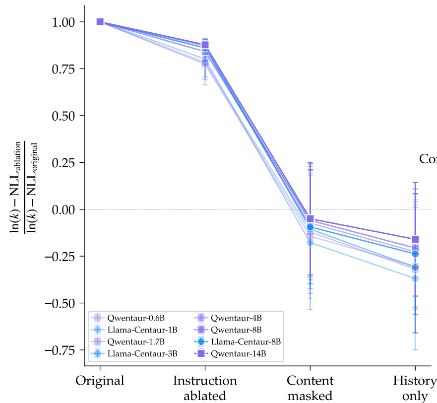
a Information retention across ablation conditions
