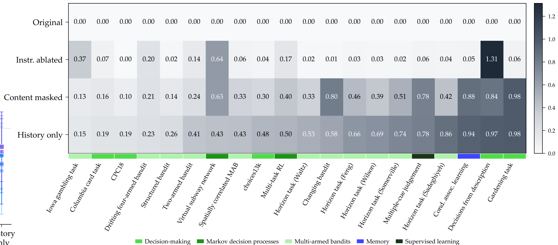
b Fraction of learned information lost by experiment
