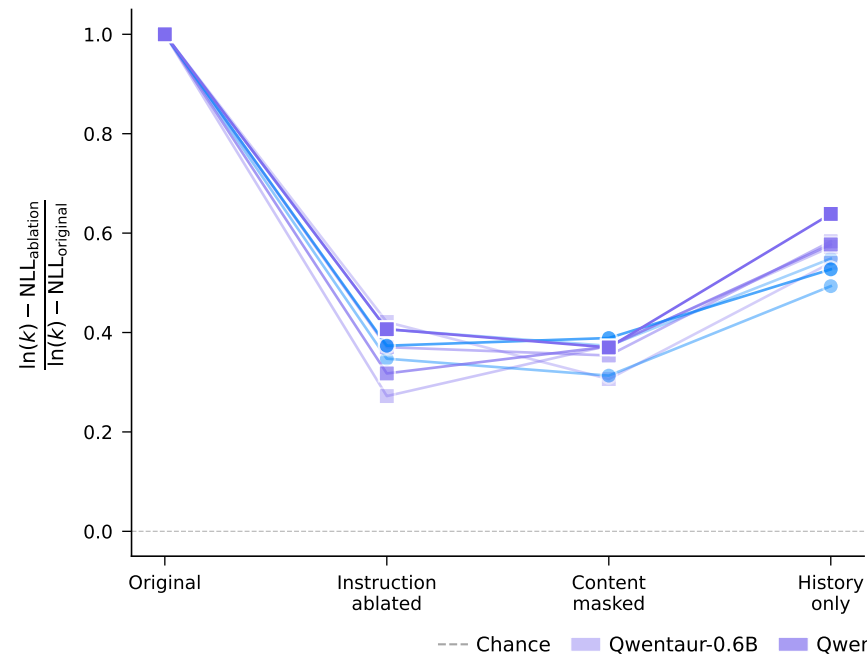
a Information retention
