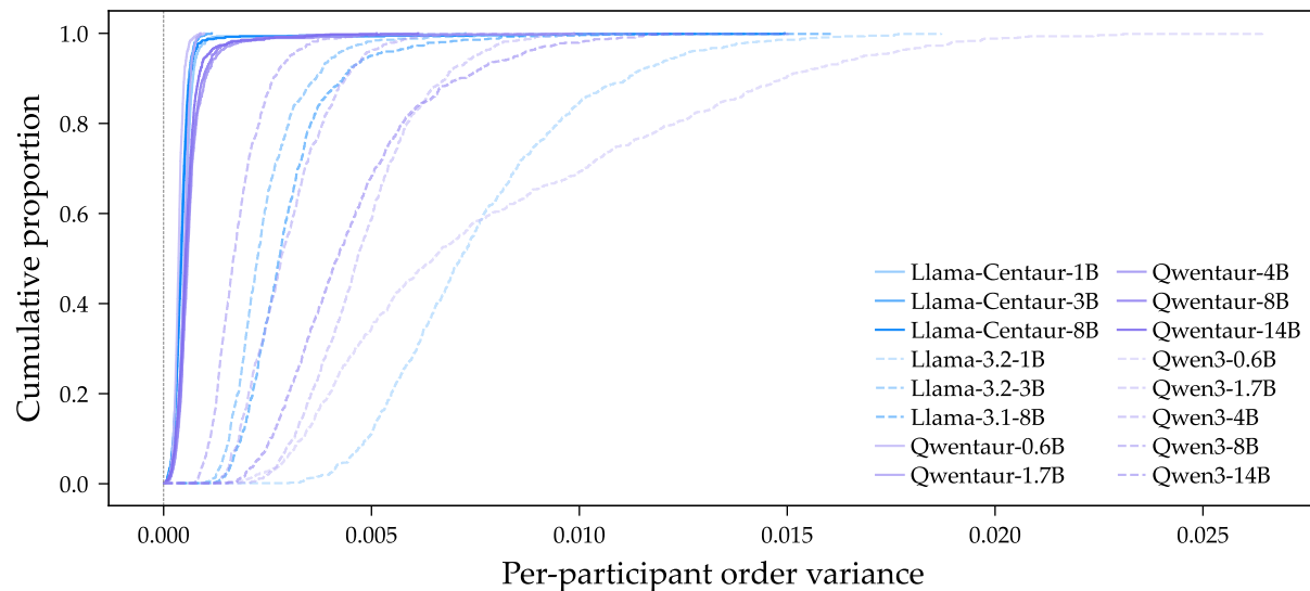
b Intertemporal choice (Ruggeri et al., 2022)
