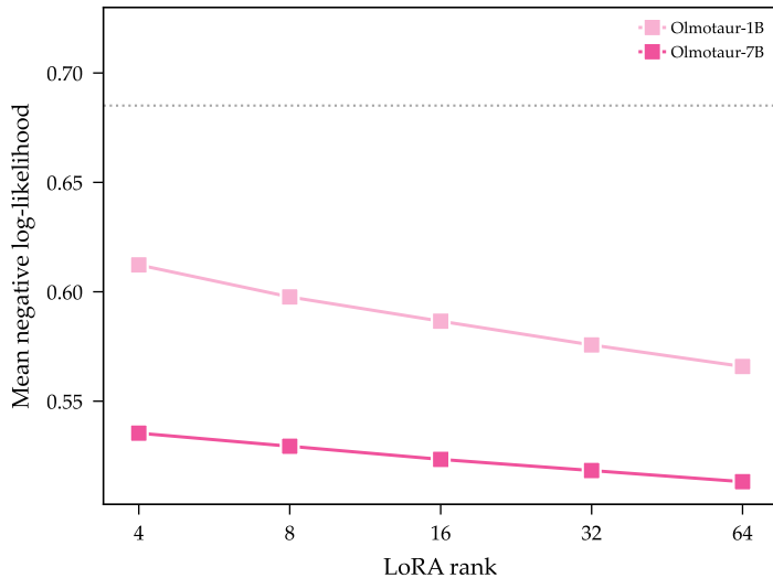
a LoRA rank sweep (full data)
