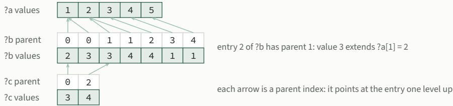
Figure 8: The three levels of the triangle join on the example, in both representations. In the row engine the number of allocations equals the number of bindings. In the batched engine it equals the number of levels.
