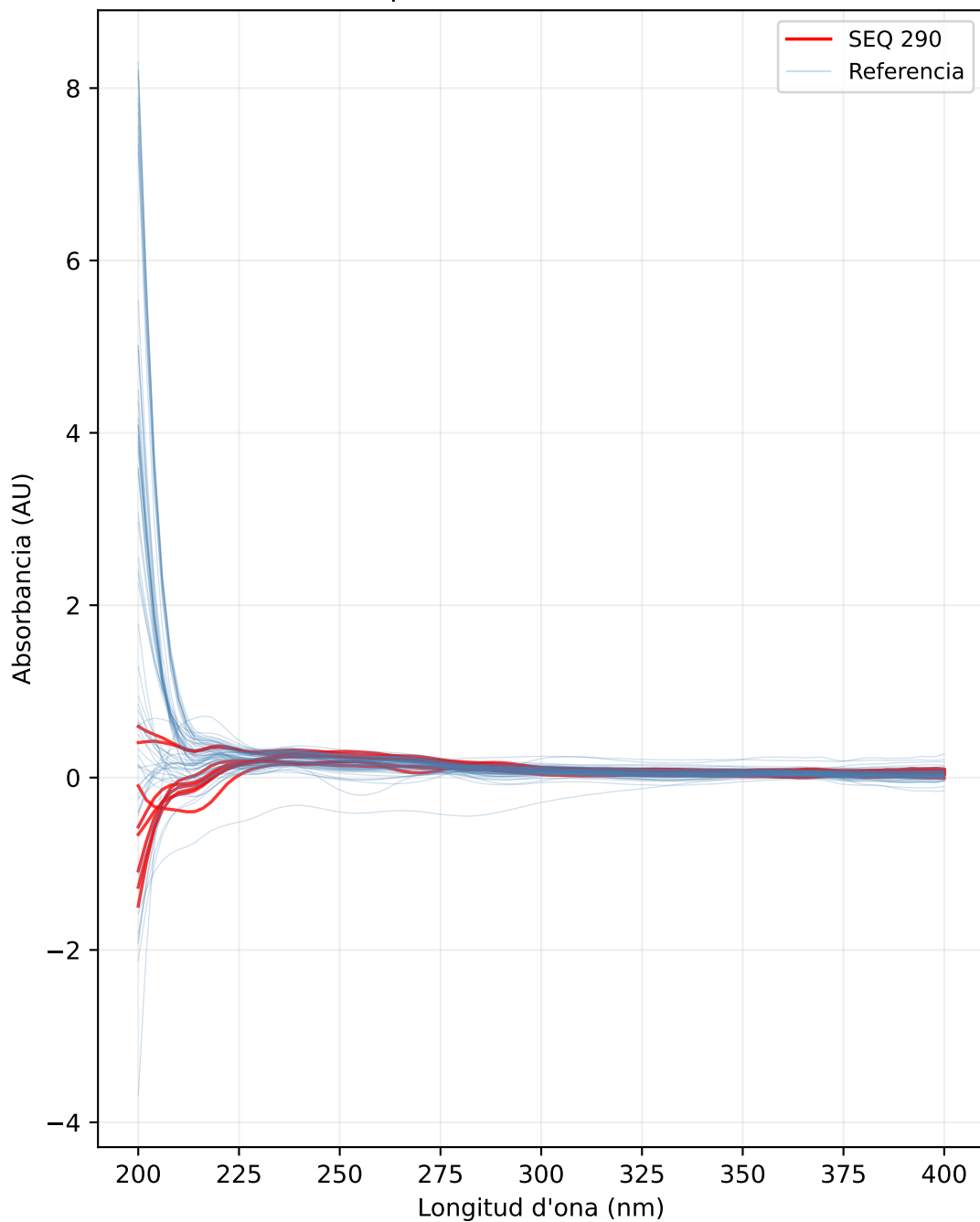
Espectre UV a t = 30 min
