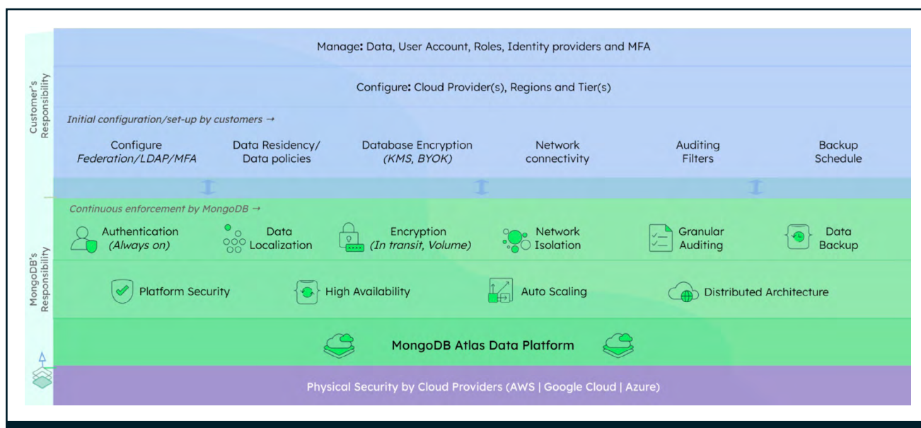
Figure 3. The MongoDB Shared Responsibility Model
