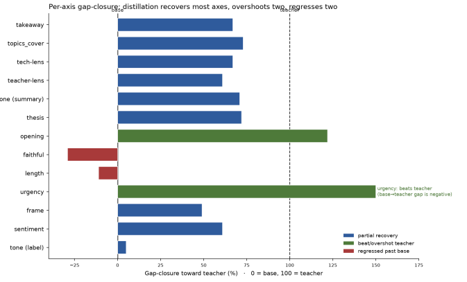
Fig. 3. Per-axis gap-closure toward the teacher (0 = untuned base, 100 = teacher). Partial recovery, overshoot, and regression below base are distinguished. Distillation recovers most summary and classification axes, overshoots two, and leaves two small summary regressions. The per-axis pattern, not any single aggregate, is the primary result.
