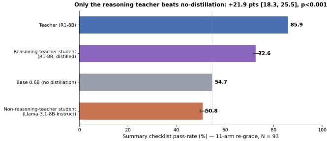
Fig. 5. Non-reasoning-teacher control (eleven-arm re-grade, N = 93 , three-seed means with seed range). Same student, recipe, seeds, and split; only the distillation teacher differs. The reasoning teacher (R1-8B) yields +21.9 checklist points over a same-size non-reasoning teacher (Llama-3.1-8B-Instruct) and is the only one of the two to beat the untuned base; the non-reasoning-teacher student is statistically level with base.
