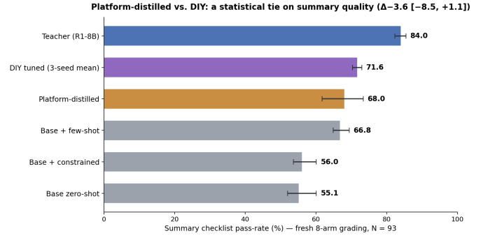
Fig. 7. Summary checklist pass-rate under the eight-arm grading (mean with bootstrap 95% interval; tuned shown as three-seed mean with seed range). The primary comparison, platform-distilled versus tuned mean, is a statistical tie.
