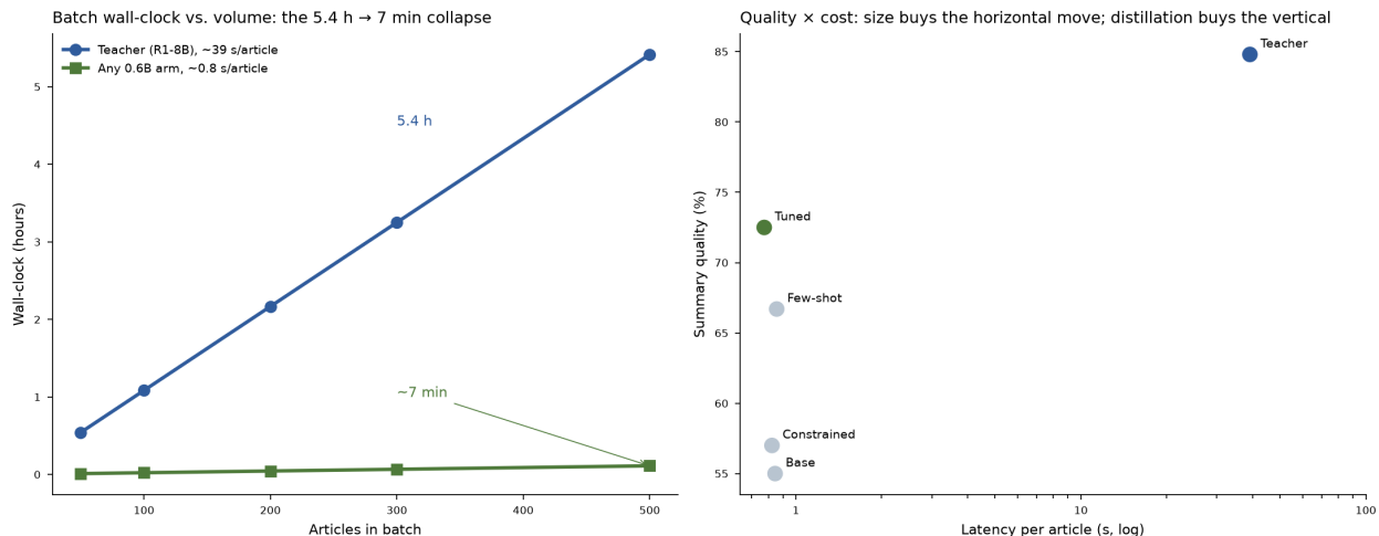
Figure 5. Left: batch wall-clock vs. volume — the 5.4 h → 7 min collapse at 500 articles that motivated the work. Right: the quality × cost plane — every 0.6B arm sits at ~0.8 s (the horizontal move is free with size); the vertical axis is where distillation, prompting, and the teacher differ, and where the tuned student beats both non-distillation controls on summary quality.
