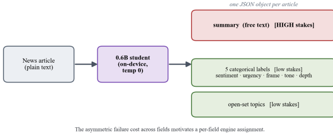
Fig. 1. The structured-enrichment task. Each article maps to one JSON object, a free-text summary, five categorical labels, and open-set topics. The failure costs are asymmetric: a hallucinated summary misleads, while a wrong label or topic is cheap. That asymmetry motivates the per-field engine assignment (Section VIII).
