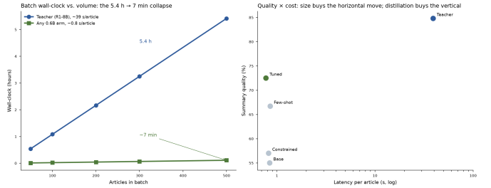
Fig. 5. Left: batch wall-clock versus volume, the 5.4 h to ~7 min collapse at 500 articles that motivated the work. Right: the quality-cost plane, every 0.6B arm sits at ~0.8 s; the vertical axis is where distillation, prompting, and the teacher differ.
