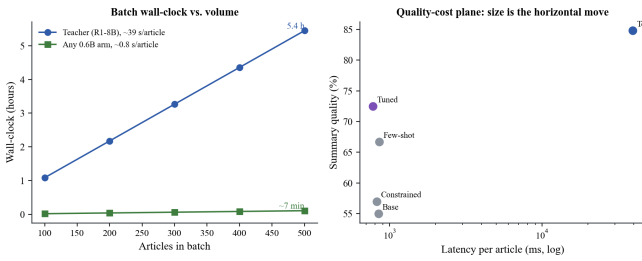
Fig. 5. Left: batch wall-clock versus volume, the 5.4 h to \sim 7 min collapse at 500 articles that motivated the work. Right: the quality-cost plane, every 0.6B arm sits at \sim 0.8 s; the vertical axis is where distillation, prompting, and the teacher differ.
