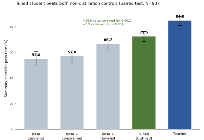
Fig. 4. Summary checklist pass-rate by arm, full-text grading, mean with bootstrap 95% interval ( N = 93 ). The tuned student significantly beats both non-distillation controls on the paired per-article test. The win rests on the paired comparison, which cancels per-article difficulty, not on marginal-interval separation.
