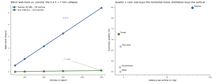
Fig. 6. Left: batch wall-clock versus volume—the 5.4 h to ~7 min collapse at 500 articles that motivated the work. Right: the quality-cost plane—every 0.6B arm sits at ~0.8 s (the horizontal move is free with size); the vertical axis is where distillation, prompting, and the teacher differ.
