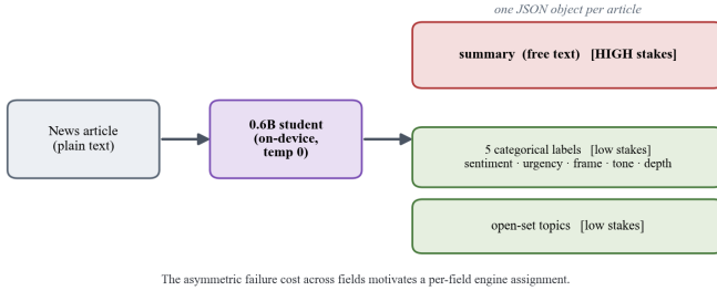
Fig. 1. The structured-enrichment task. Each article maps to one JSON object—a free-text summary, five categorical labels, and open-set topics. The failure costs are asymmetric: a hallucinated summary misleads, while a wrong label or topic is cheap. That asymmetry motivates the per-field engine assignment (Section VIII).
