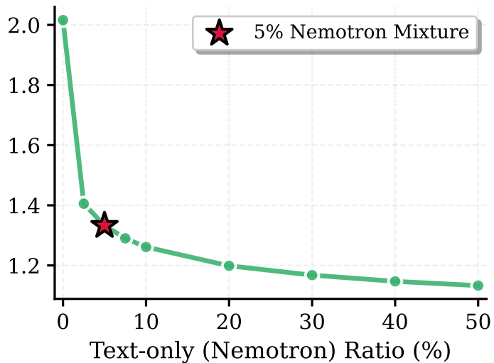
Valid Loss on Paloma (C4-en) in bpb
