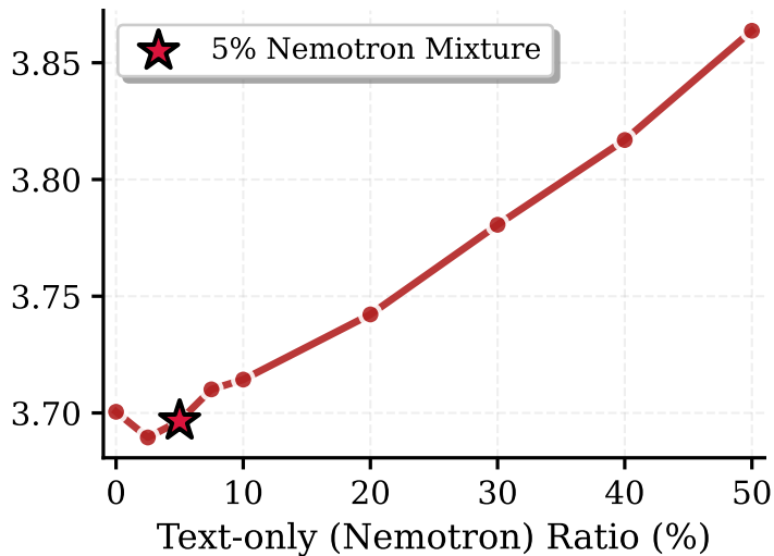
Valid Loss on LibriSpeech
