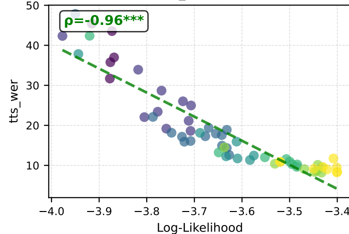
swuggy (↑)
