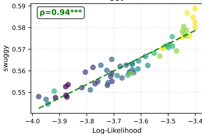
swuggy (↑)
