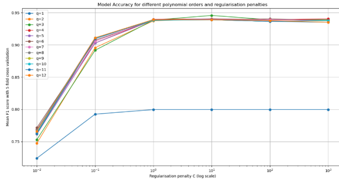
Figure 5: Model F1 scores at different max polynomial orders and regularization penalty
