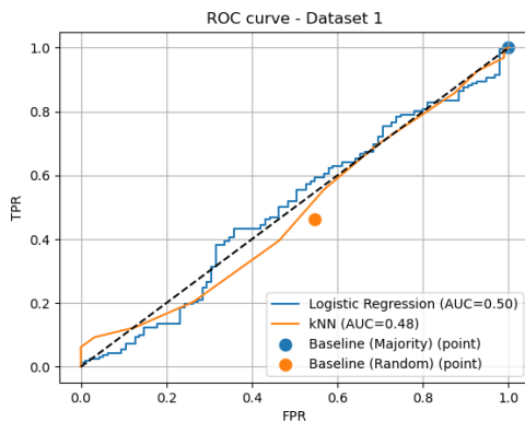
Figure 4: ROC curve for Logistic Regression and kNN and points outlining 2 baseline models (pick randomly and choose most frequent class)
