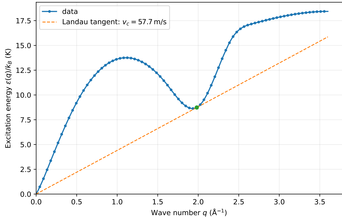
Dispersion relation of superfluid helium
