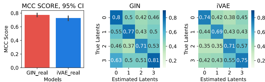
Figure 9: MCC scores and mean correlation matrices of GIN and iVAE matched with the best permutation for the setting of Fig. 1c.
