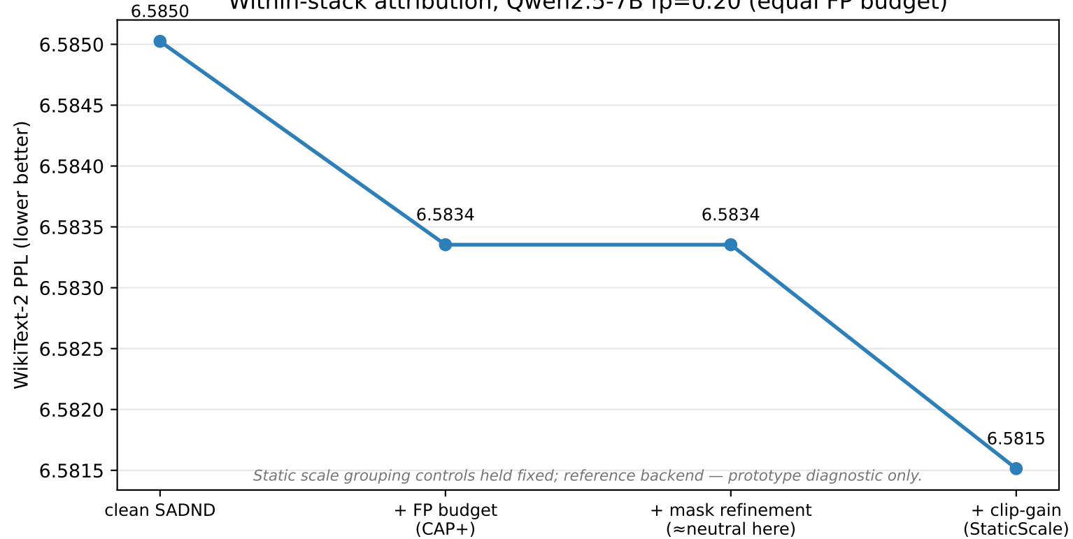
Within-stack attribution, Qwen2.5-7B fp=0.20 (equal FP budget)
