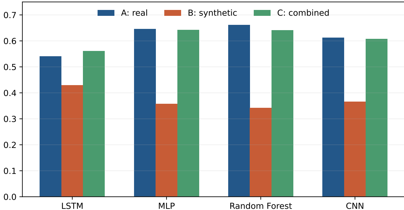
Mean macro-F1 across CWEs
