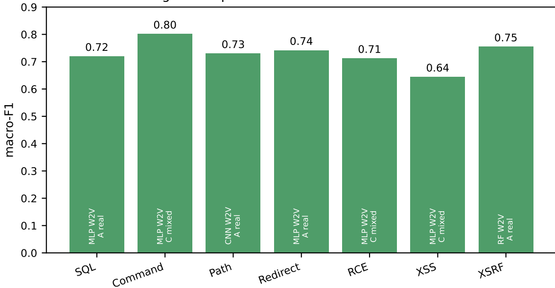
Best configuration per CWE on held-out real VUDENC windows
