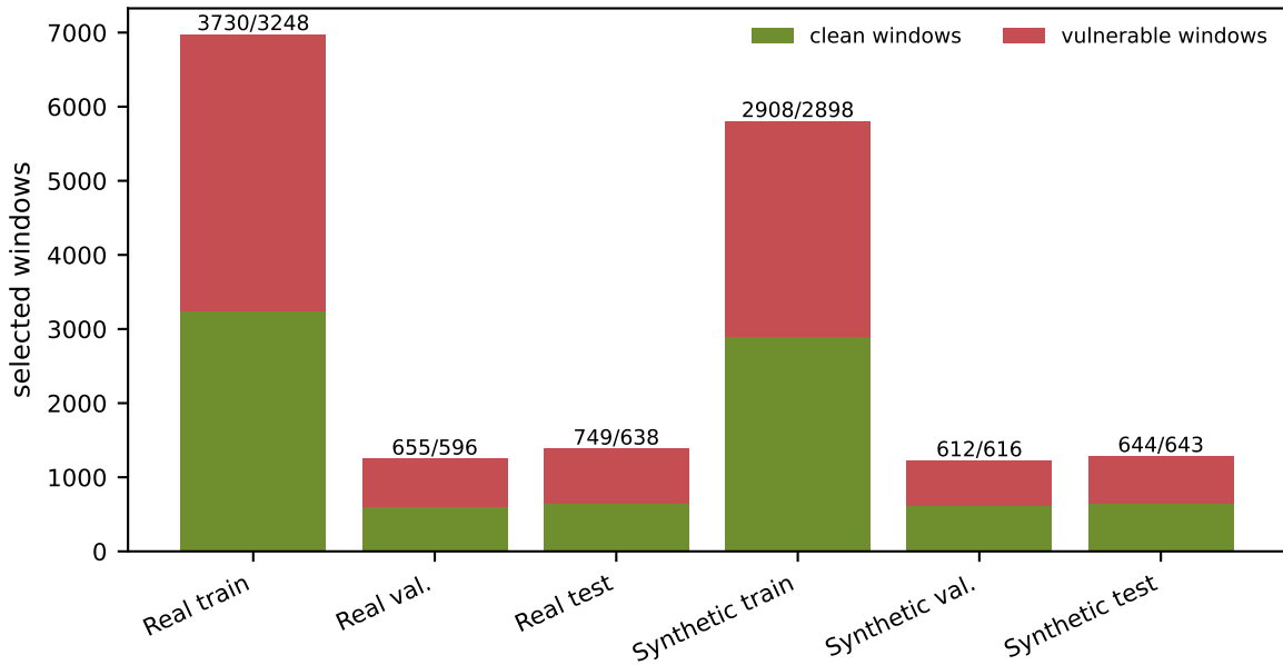
Window labels after commit-level splitting
