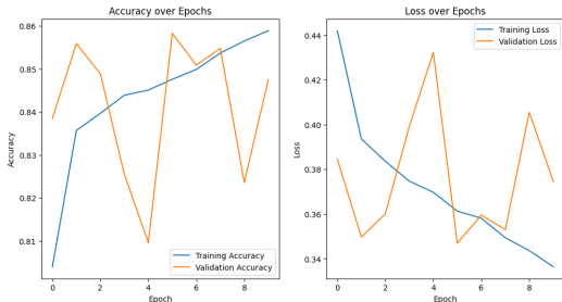
Figure 1: Training and validation per epoch
