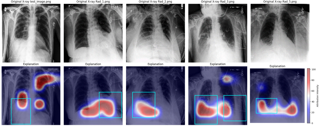
Figure 2: GradCAM Explanations
