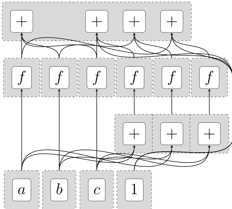
Figure 2.2: EMT of the term f(a) + f(b) + f(c) after some steps.
