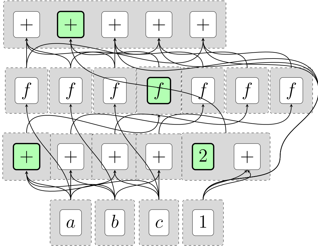
Figure 2.3: EMT of the term f(a) + f(b) + f(c) once saturated, highlighting the desired term.
