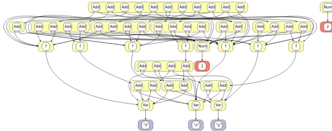
Figure 13: E-graph at timeout
