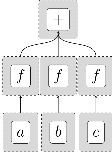
Figure 2.2: EMT of the term f(a) + f(b) + f(c) after some steps.
