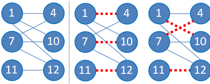
Figure 4.37: Bipartite Matching problem
