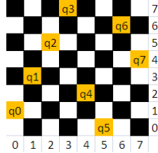
Figure 3.1: 8-Queens
