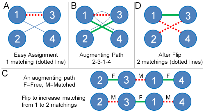
Figure 4.38: Augmenting Path Algorithm
