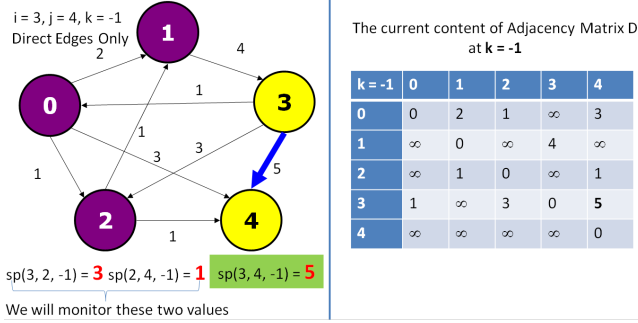
Figure 4.23: Floyd-Warshall Explanation 1
