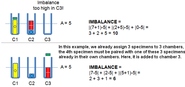
Figure 3.8: UVa 00410 - Observations
