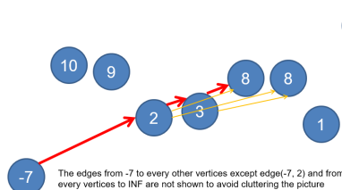
Figure 4.43: LIS as Longest Path of an Implicit DAG; Also See Figure 3.13
