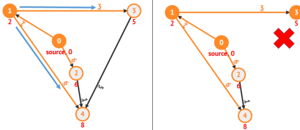
Figure 4.17: Dijkstra's Animation, Steps 3+4
