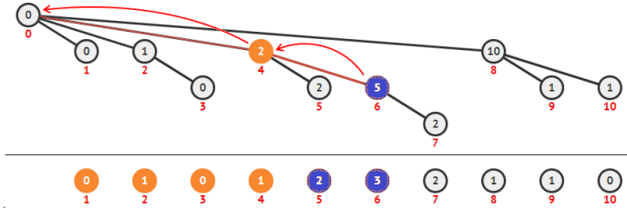
Figure 2.12: Example of rsq(6) on Fenwick (Interrogation/Query) Tree
