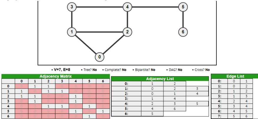
Figure 2.7: Graph Data Structure Visualization, Undirected/Unweighted Graph
