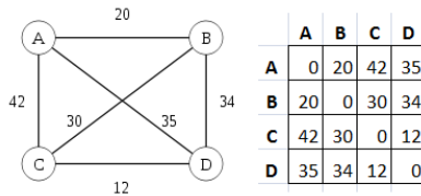
Figure 3.15: A Complete Weighted Graph K_4
