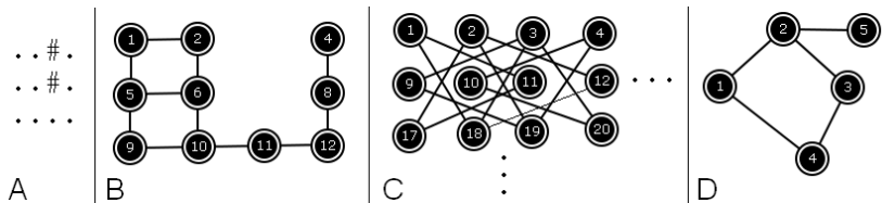
Figure 2.8: Implicit Graph Examples
