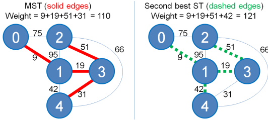
Figure 4.14: Second Best ST (from UVa 10600 [44])
