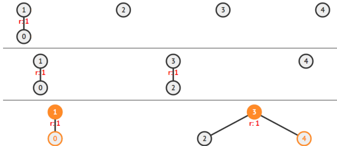
Figure 2.11: unionSet(0, 1) → (2, 3) → (4, 3) and isSameSet(0, 4)
