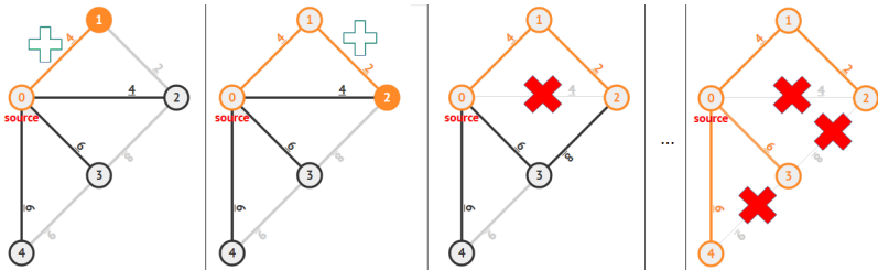
Figure 4.11: Animation of Prim's Algorithm for the same graph as in Figure 4.9—left
