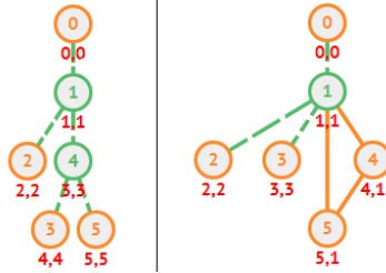
Figure 4.6: Finding Articulation Points with dfs_num and dfs_low
