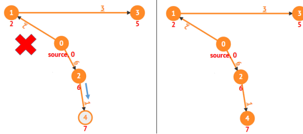
Figure 4.18: Dijkstra's Animation, Steps 5+6
