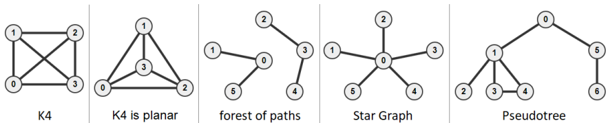
Figure 4.41: A Few Other Special Graphs
