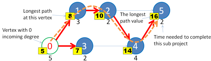
Figure 4.29: The Longest Path on this DAG
