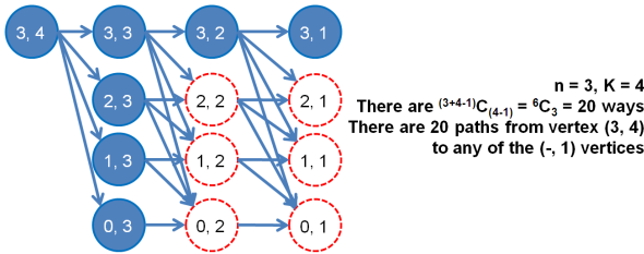
Figure 4.35: UVa 10943 as Counting Paths in DAG
