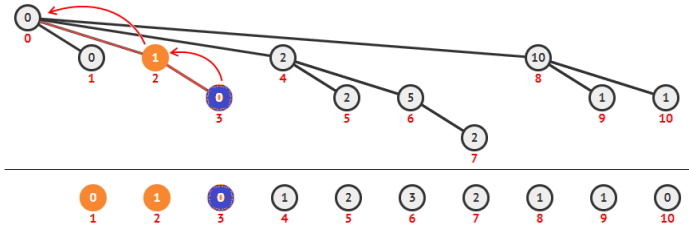
Figure 2.13: Example of \text{rsq}(3) on Fenwick (Interrogation/Query) Tree
