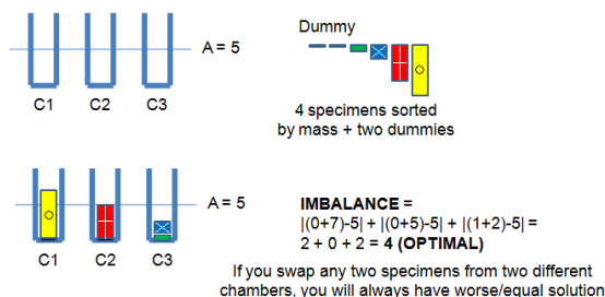
Figure 3.9: UVa 00410 - Greedy Solution
