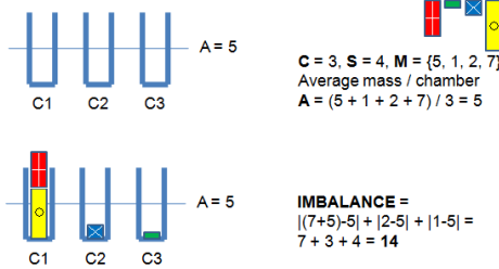
Figure 3.7: Visualization of UVa 00410 - Station Balance
