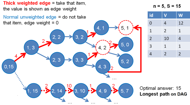
Figure 4.34: 0-1 KNAPSACK as Longest Paths on DAG
