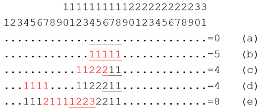
Figure 2.17: RURQ Example; Range Queries are Underlined
