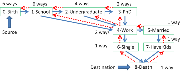
Figure 4.31: Example of Counting Paths in DAG - Top-Down
