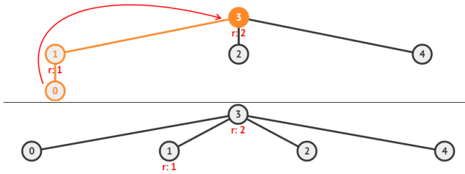
Figure 2.10: Top: findSet(0) , Bottom: The Subsequent Path Compression
