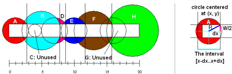
Figure 3.10: Kattis - grass/UVa 10382 - Watering Grass
