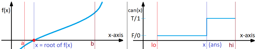
Figure 3.5: Monotone Function; Left: Bisection; Right: BSTA
