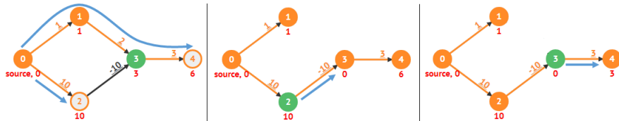
Figure 4.20: Modified Dijkstra's Can Work on a Non-Negative Cycle Graph, s = 0
