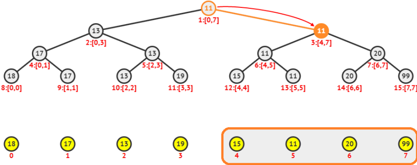
Figure 2.20: Segment Tree of A = \{18, 17, 13, 19, 15, 11, 20, \infty\} and \text{RMQ}(4, 7) = 11
