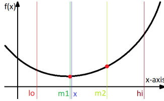
Figure 3.6: Ternary Search on a Unimodal Function
