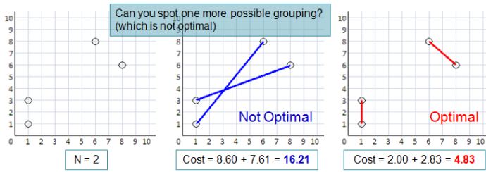
Figure 1.1: Illustration of UVa 10911 - Forming Quiz Teams
