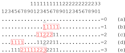
Figure 2.15: RUPQ Example; Point Queries i = 14 are Underlined
