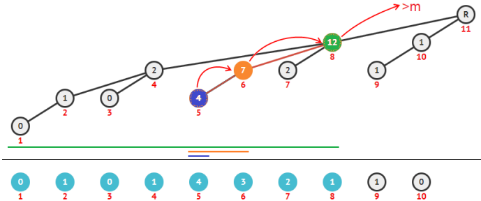
Figure 2.14: Example of \text{update}(5, 2) on Fenwick (Updating) Tree
