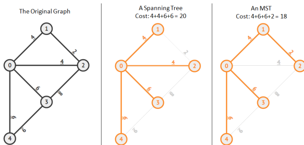
Figure 4.9: Example of an MST Problem
