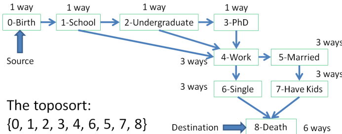
Figure 4.30: Example of Counting Paths in DAG - Bottom-Up
