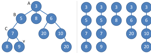
Figure 3.4: My Ancestor (all 5 root-to-leaf paths are sorted)
