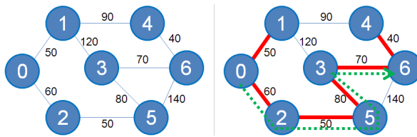
Figure 4.13: Minimax (UVa 10048 [44])
