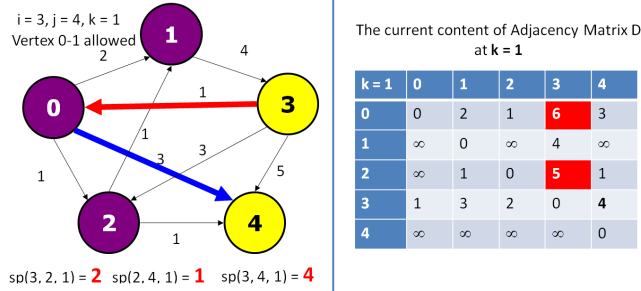
Figure 4.25: Floyd-Warshall Explanation 3
