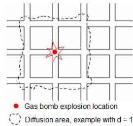
Figure 3.3: UVa 10360 [44]
