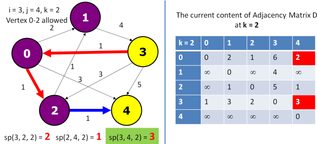
Figure 4.26: Floyd-Warshall Explanation 4
