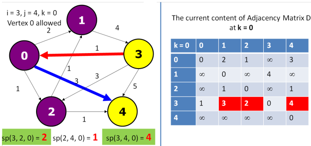
Figure 4.24: Floyd-Warshall Explanation 2
