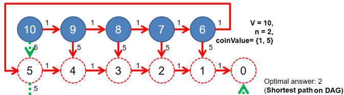
Figure 4.33: COIN-CHANGE as Shortest Paths on DAG
