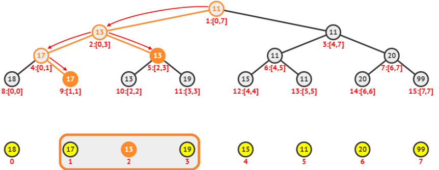
Figure 2.19: Segment Tree of A = \{18, 17, 13, 19, 15, 11, 20, \infty\} and \text{RMQ}(1, 3) = 13
