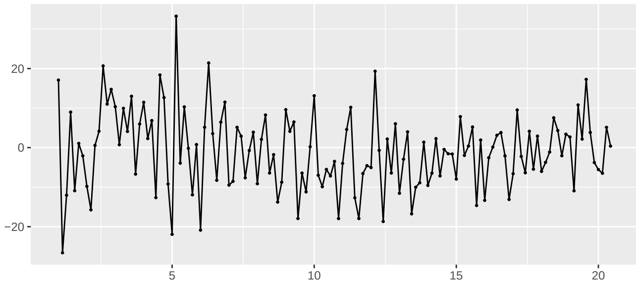
Residuals from Simple exponential smoothing
