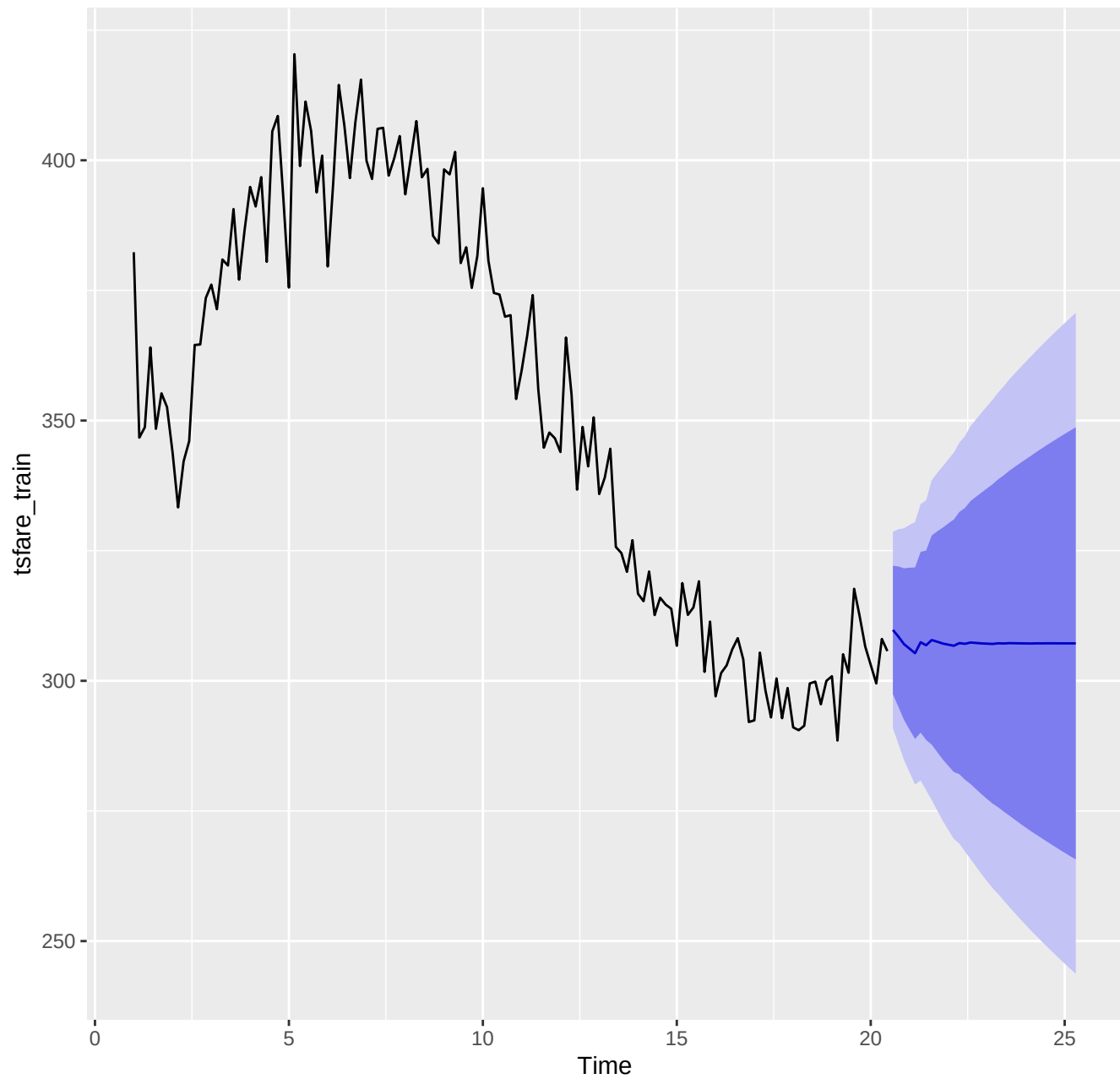
SARIMA Forecast with Confidence Intervals
