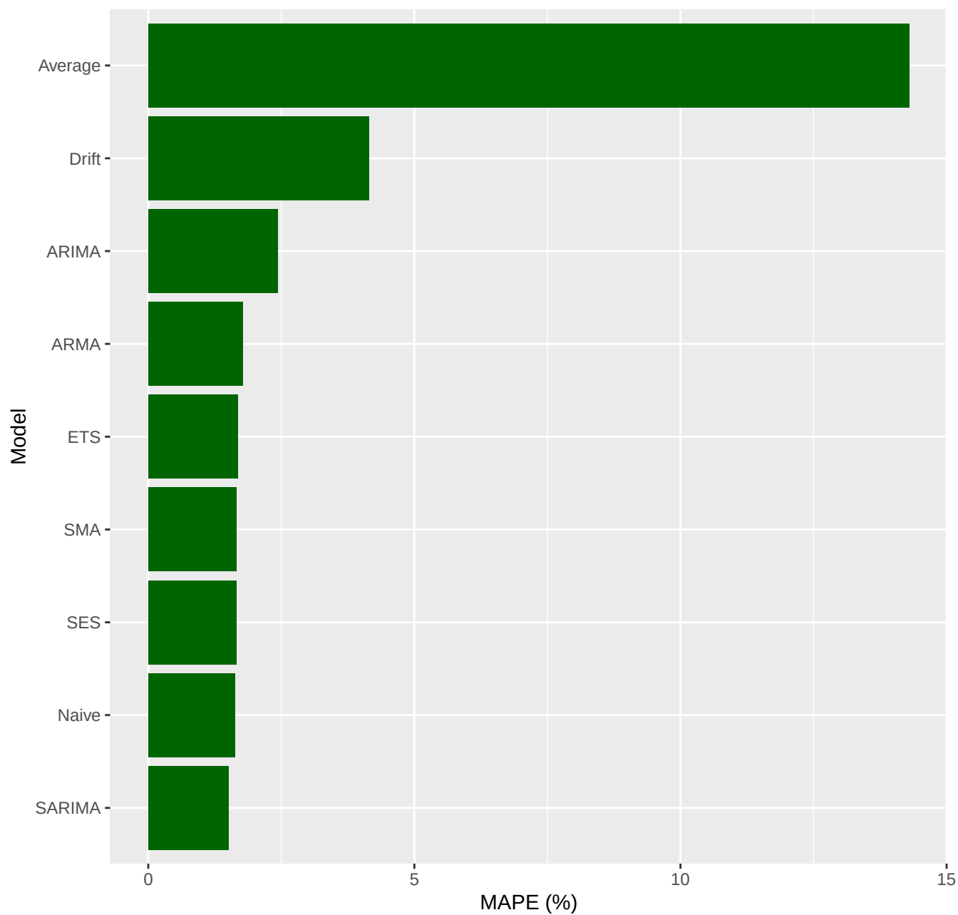
Model Comparison – MAPE (Lower is Better)
