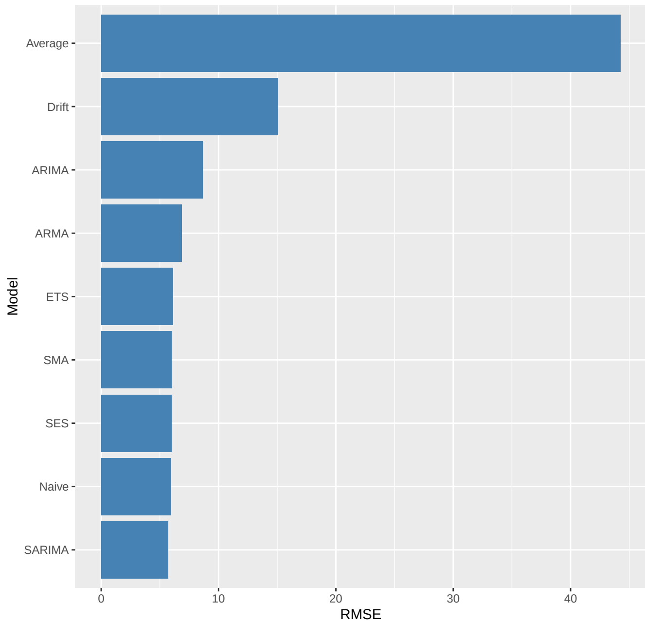
Model Comparison – RMSE (Lower is Better)
