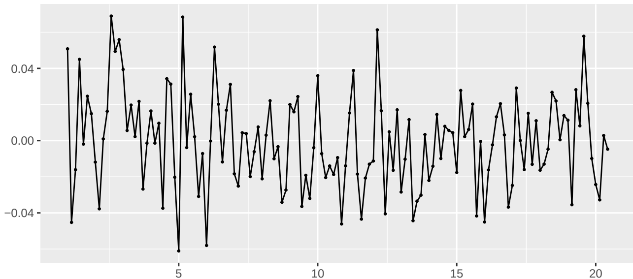
Residuals from ETS(M,Ad,N)
