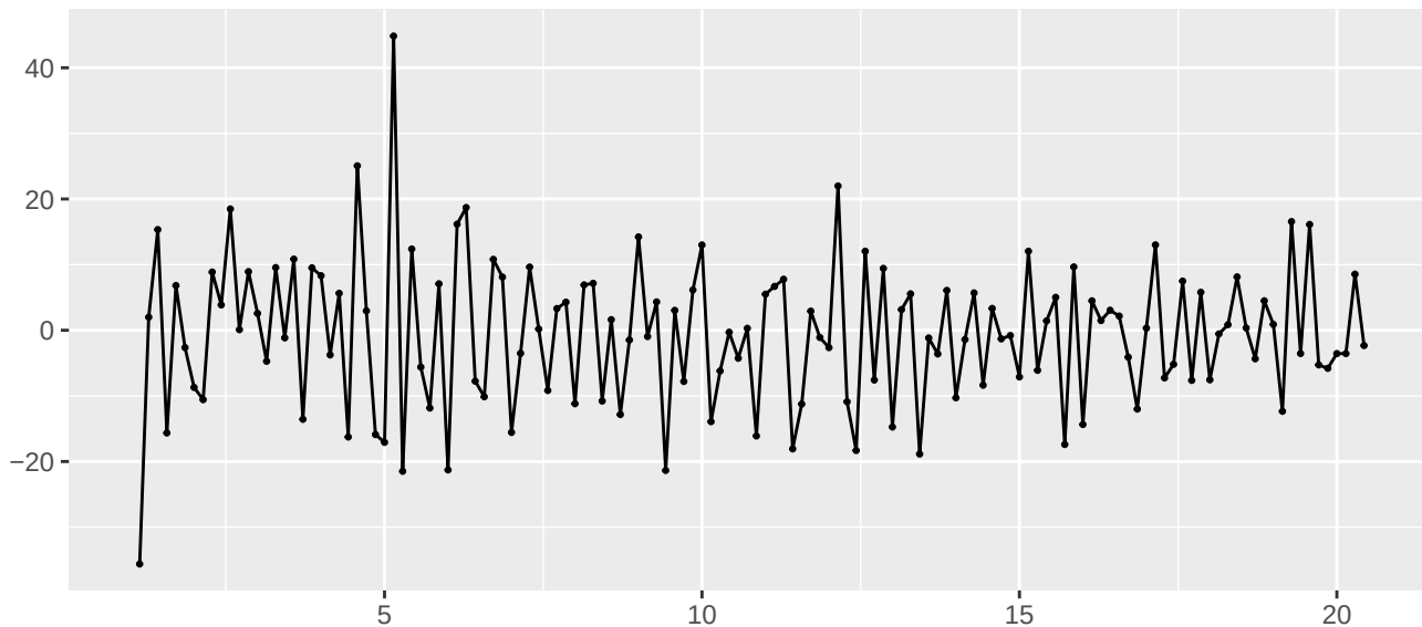
Residuals from Naive method
