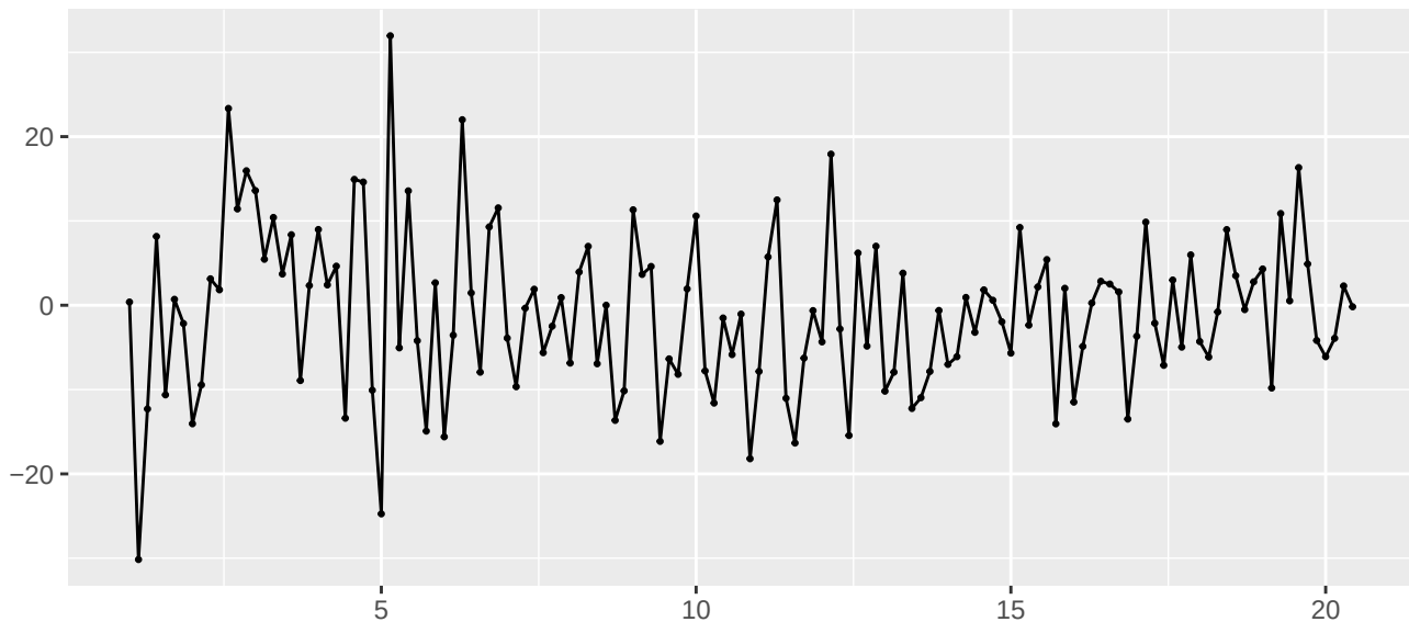
Residuals from ARIMA(0,1,1)(1,0,0)[7]
