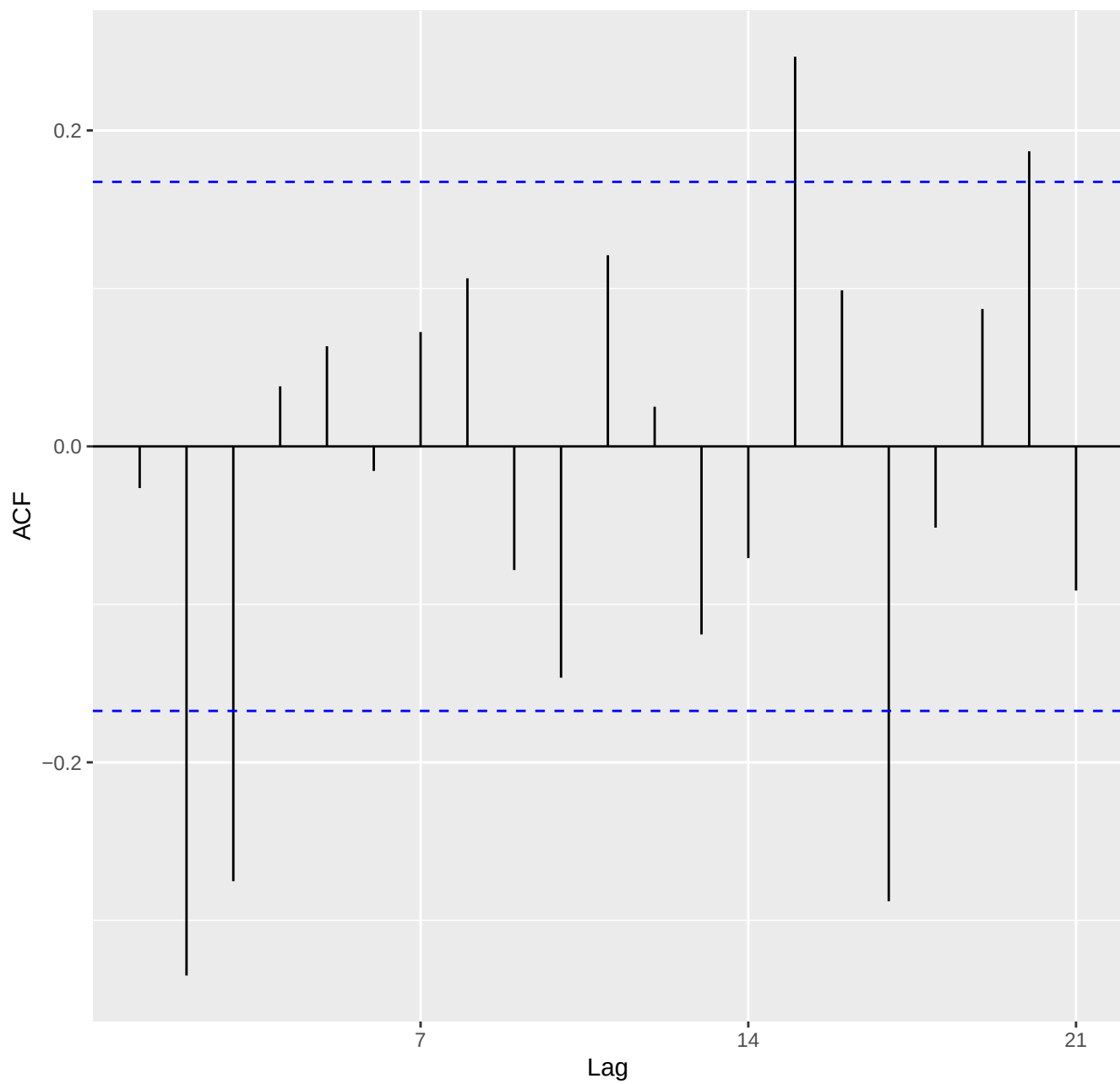
Series: fare.decomp$random
