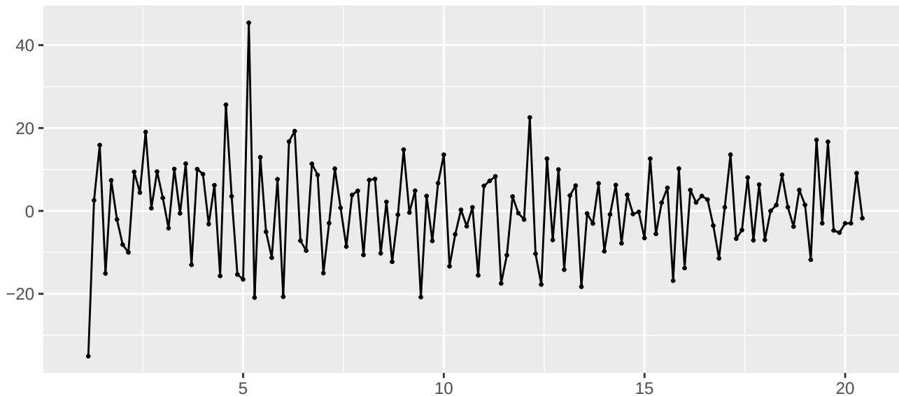
Residuals from Random walk with drift
