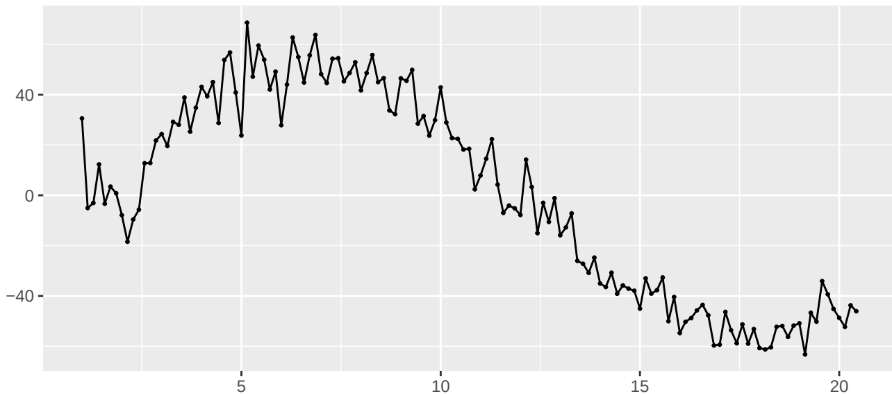
Residuals from Mean
