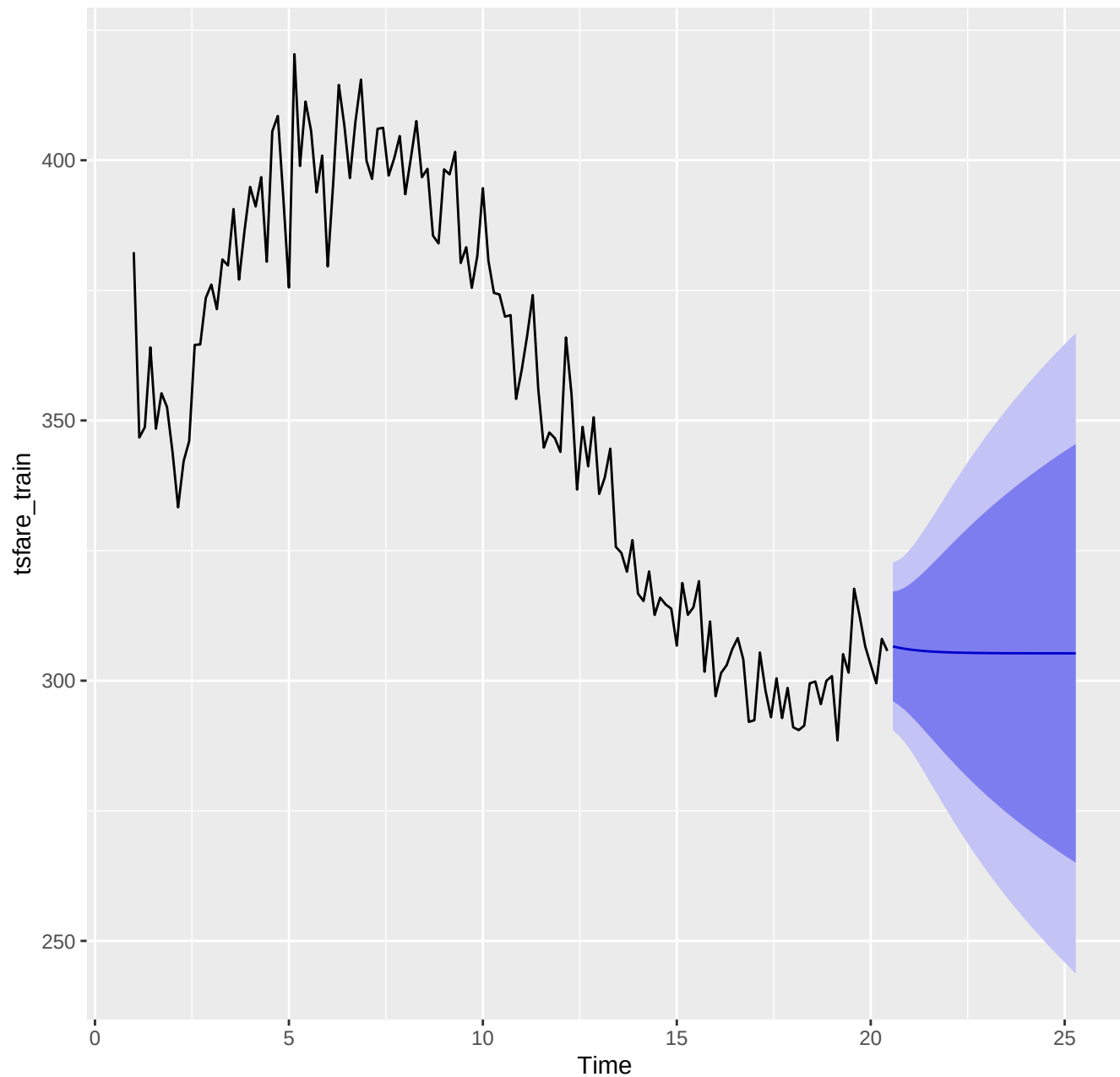
Forecasts from ETS(M,Ad,N)
