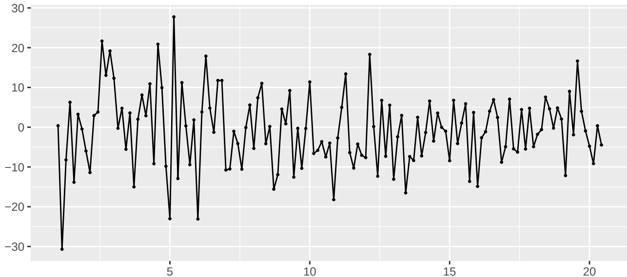
Residuals from ARIMA(2,1,2)
