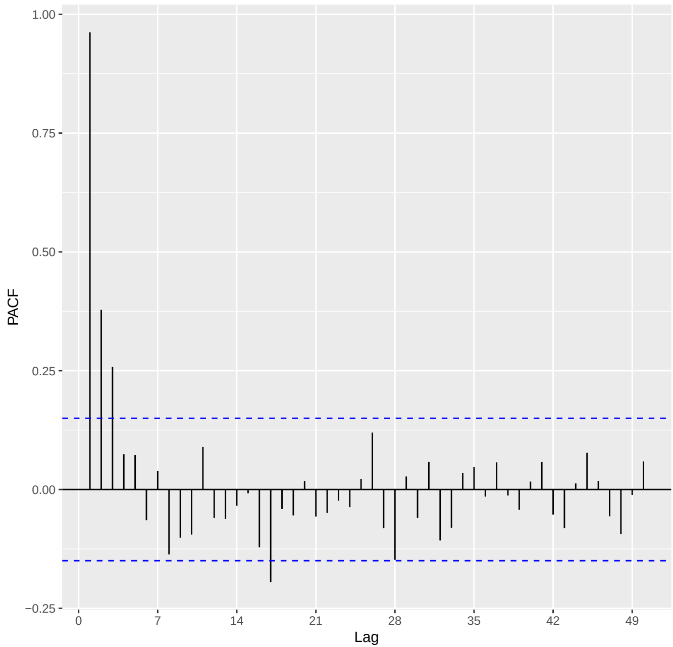
Series: tsfare
