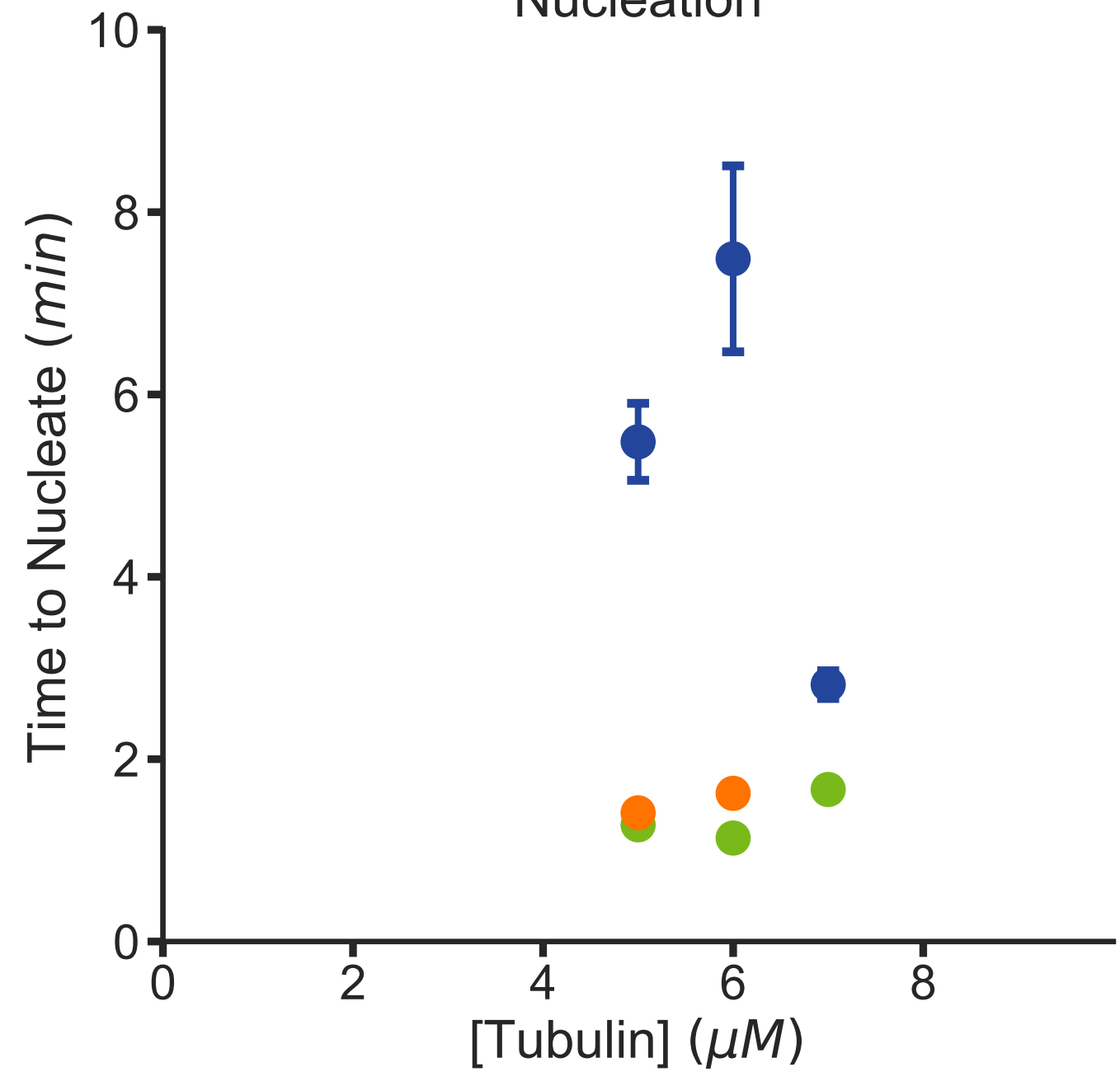
Nucleation
