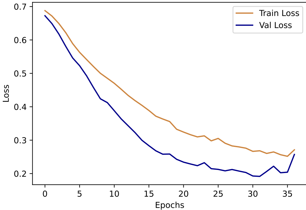
Binary Classification Loss
